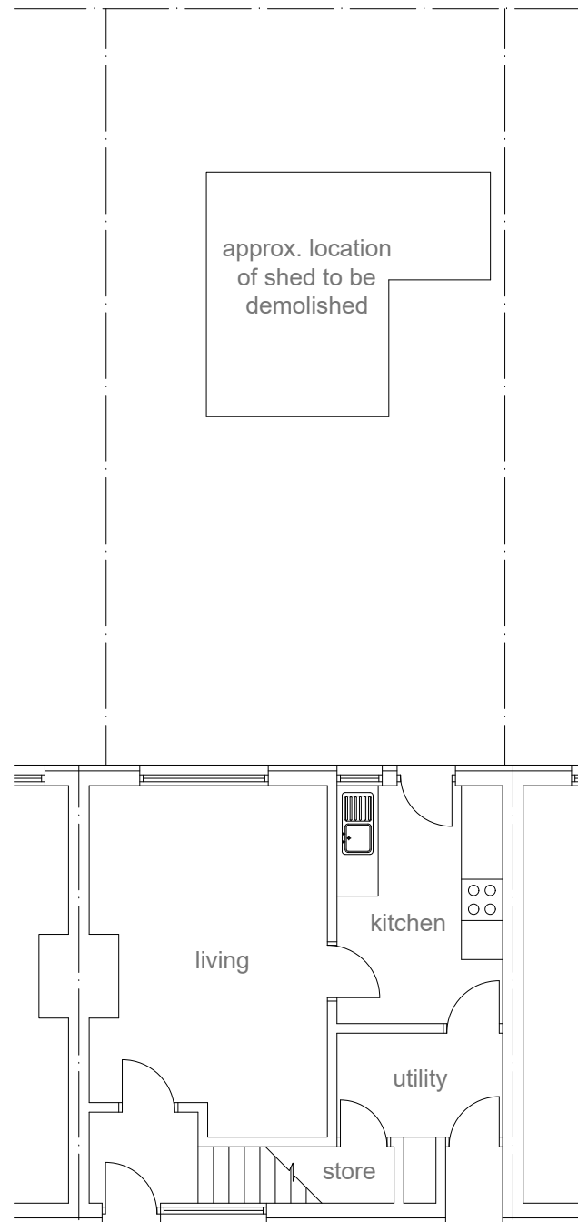
Existing ground floor and site plan @ 1:100 scale
