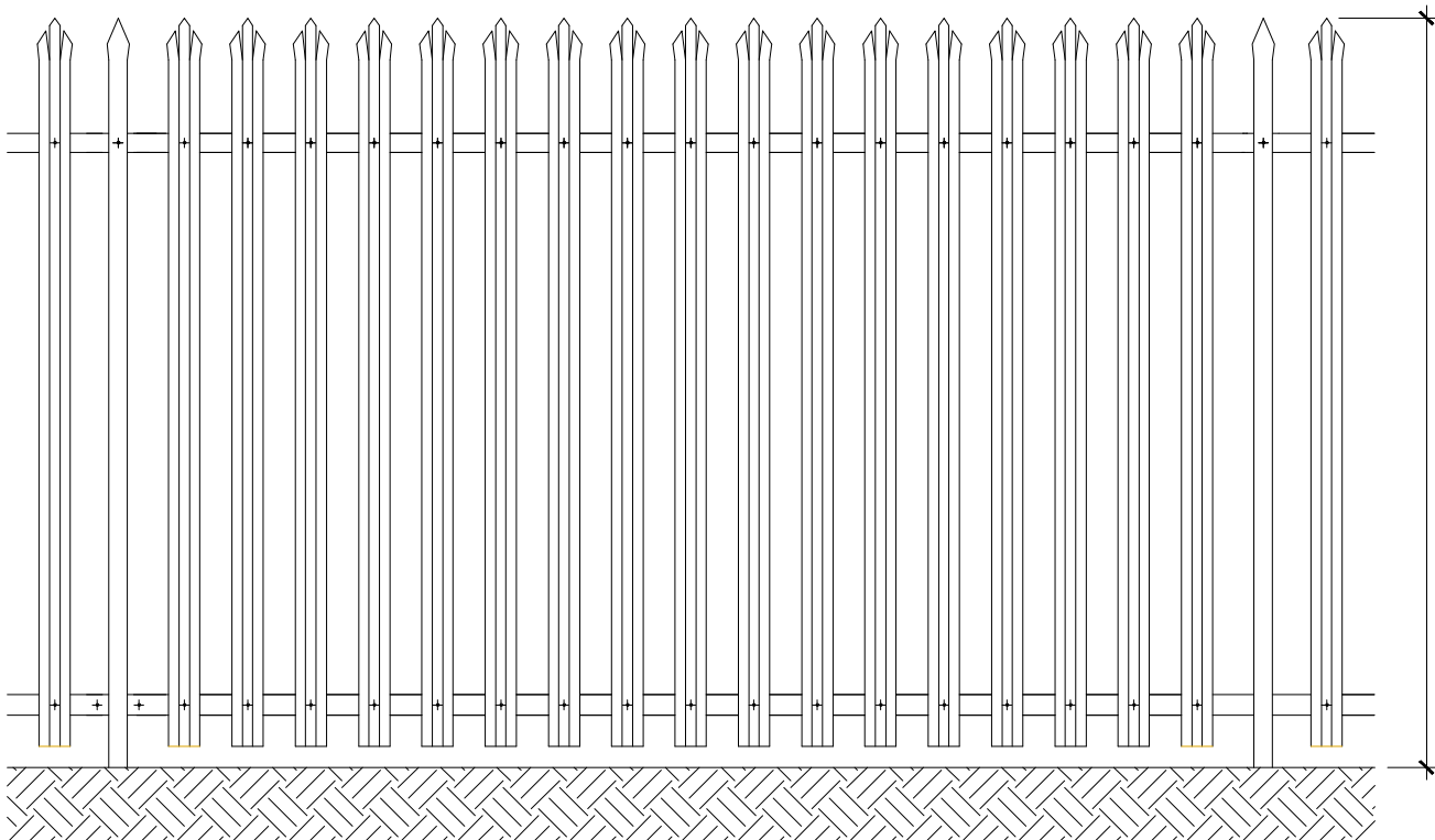
TYPICAL PALISADE FENCE DETAILS SCALE 1:20
