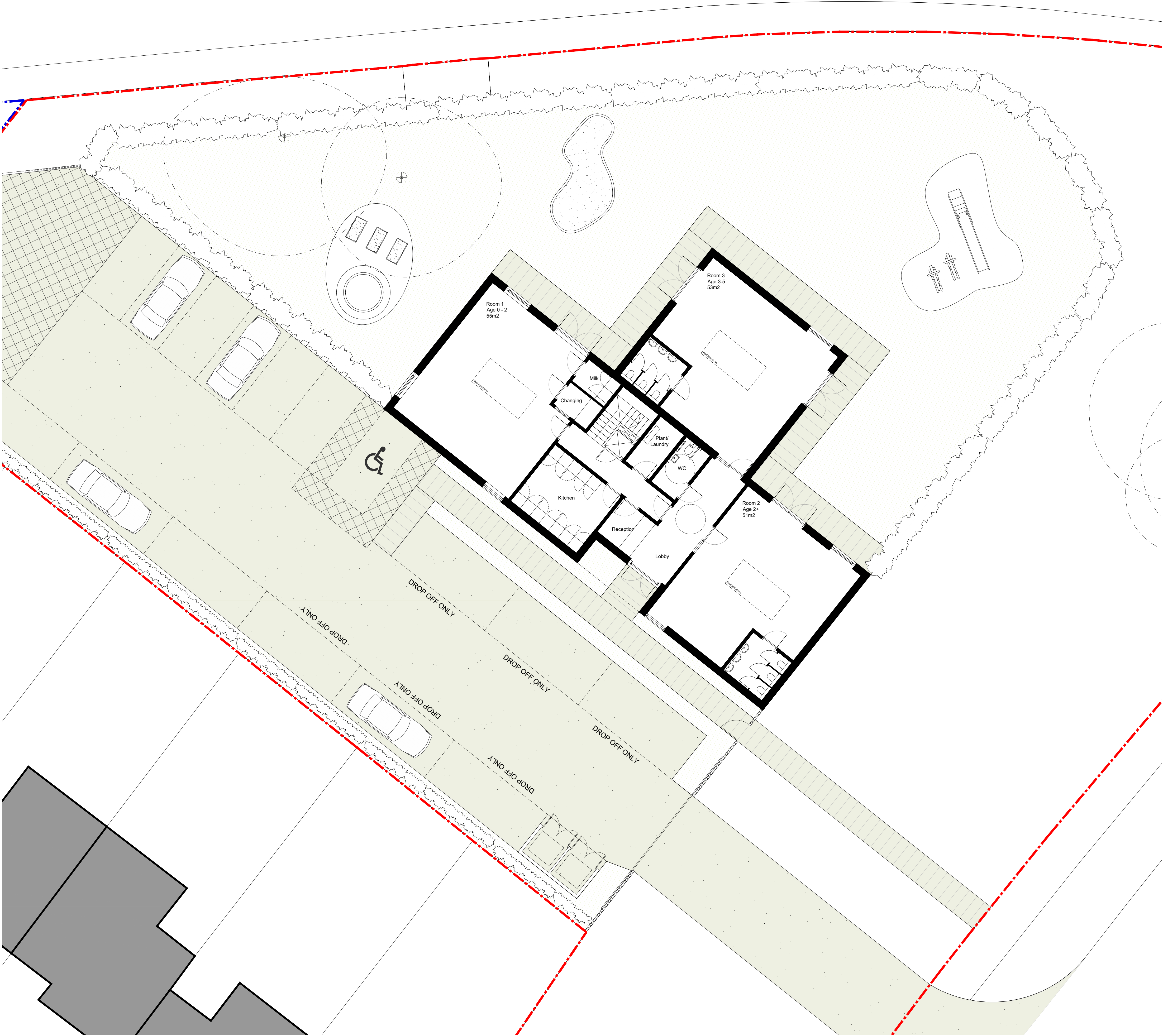
Proposed Ground Floor - In Context Scale 1:100
