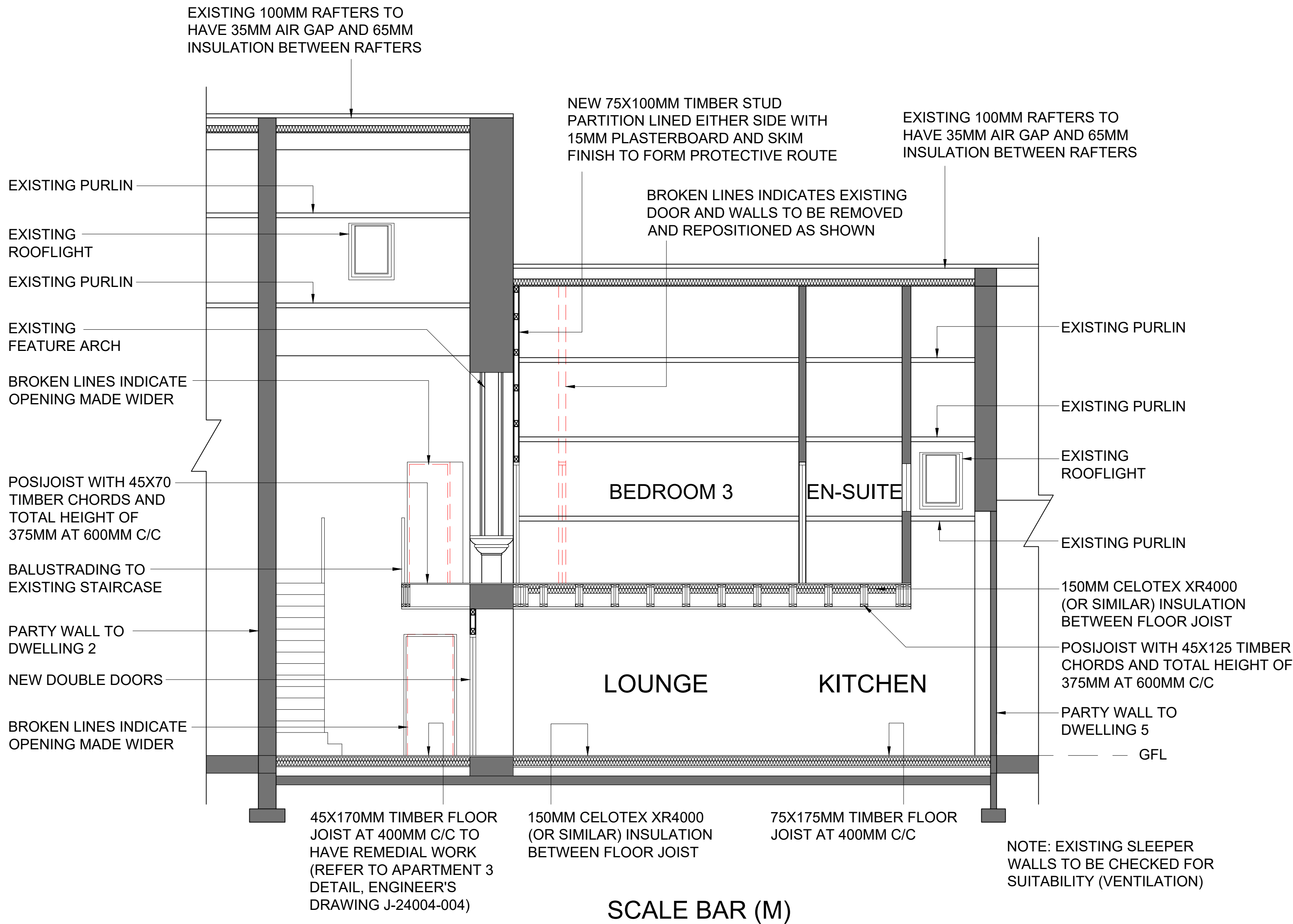
PROPOSED SECTION G-G
