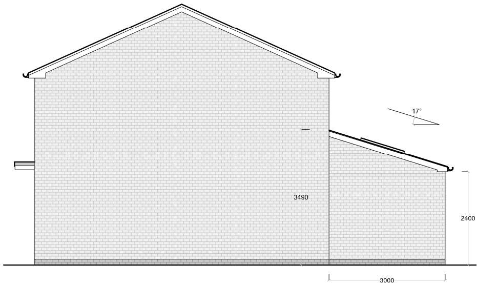
PROPOSED SIDE ELEVATION (Scale 1:100) SCALE BAR - (mm) 500 1000 2000
