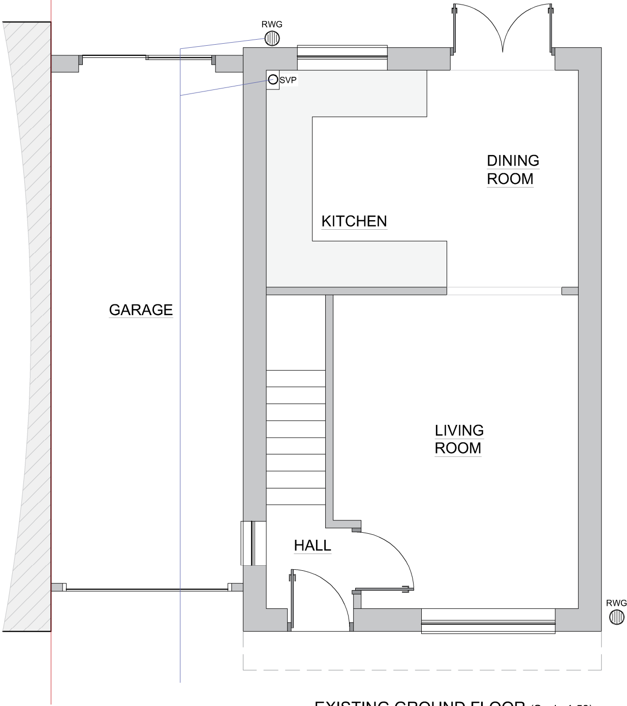
EXISTING GROUND FLOOR (Scale 1:50)
