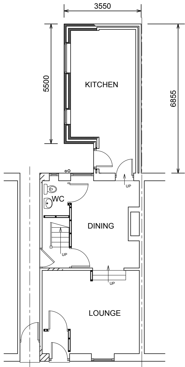
GROUND FLOOR PLAN AS PROPOSED
