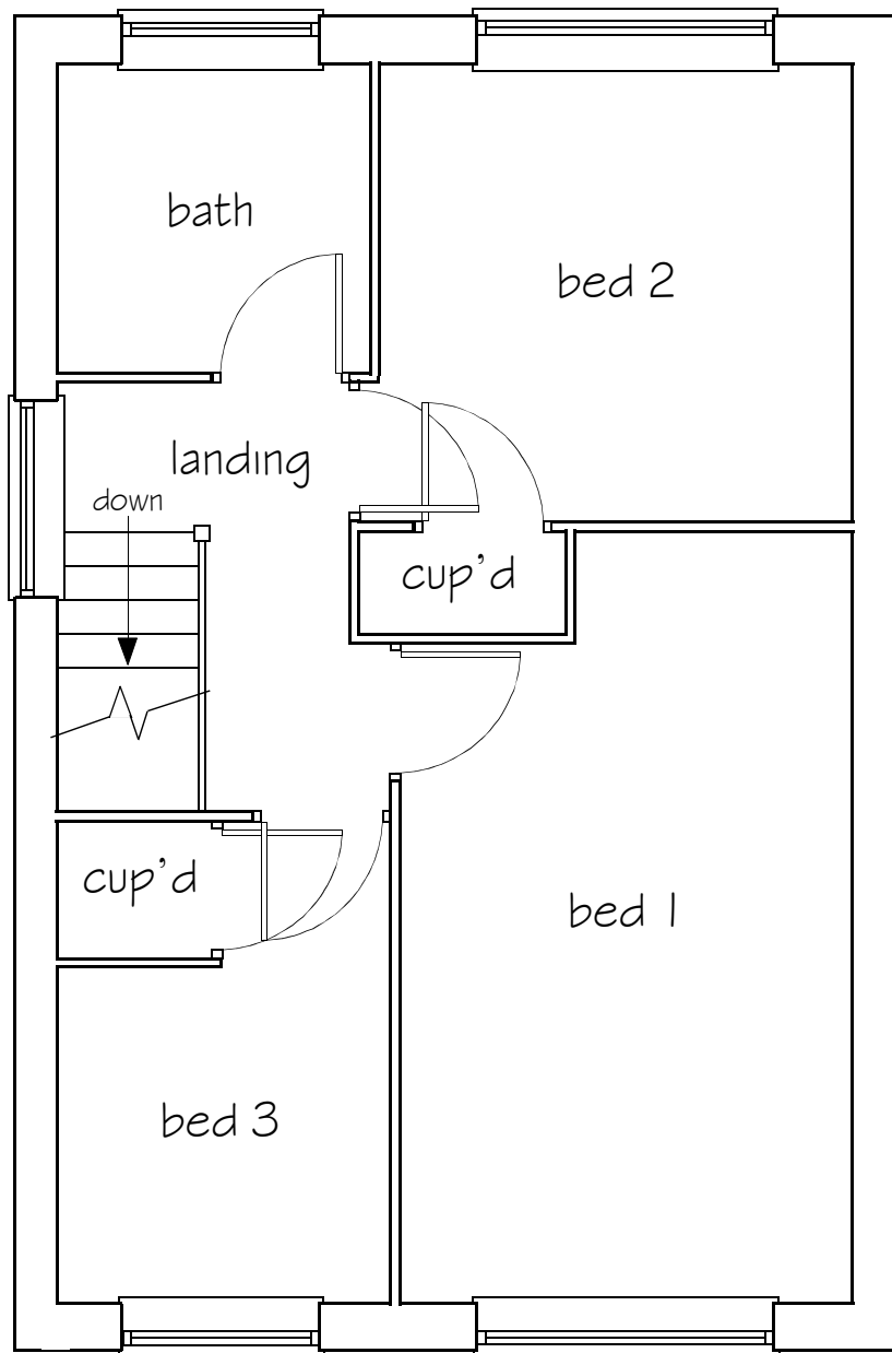
FIRST FLOOR (existing)
