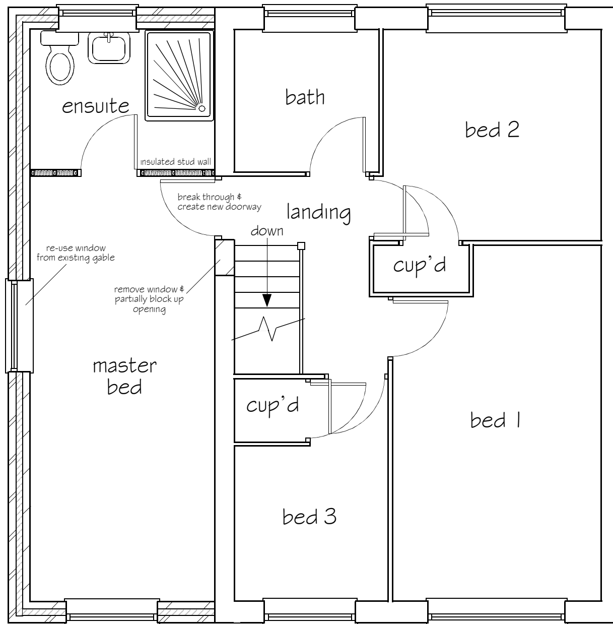
FIRST FLOOR (proposed)
