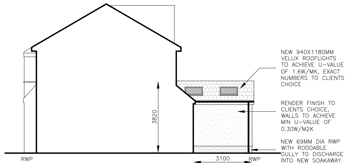
PROPOSED SIDE B ELEVATION
