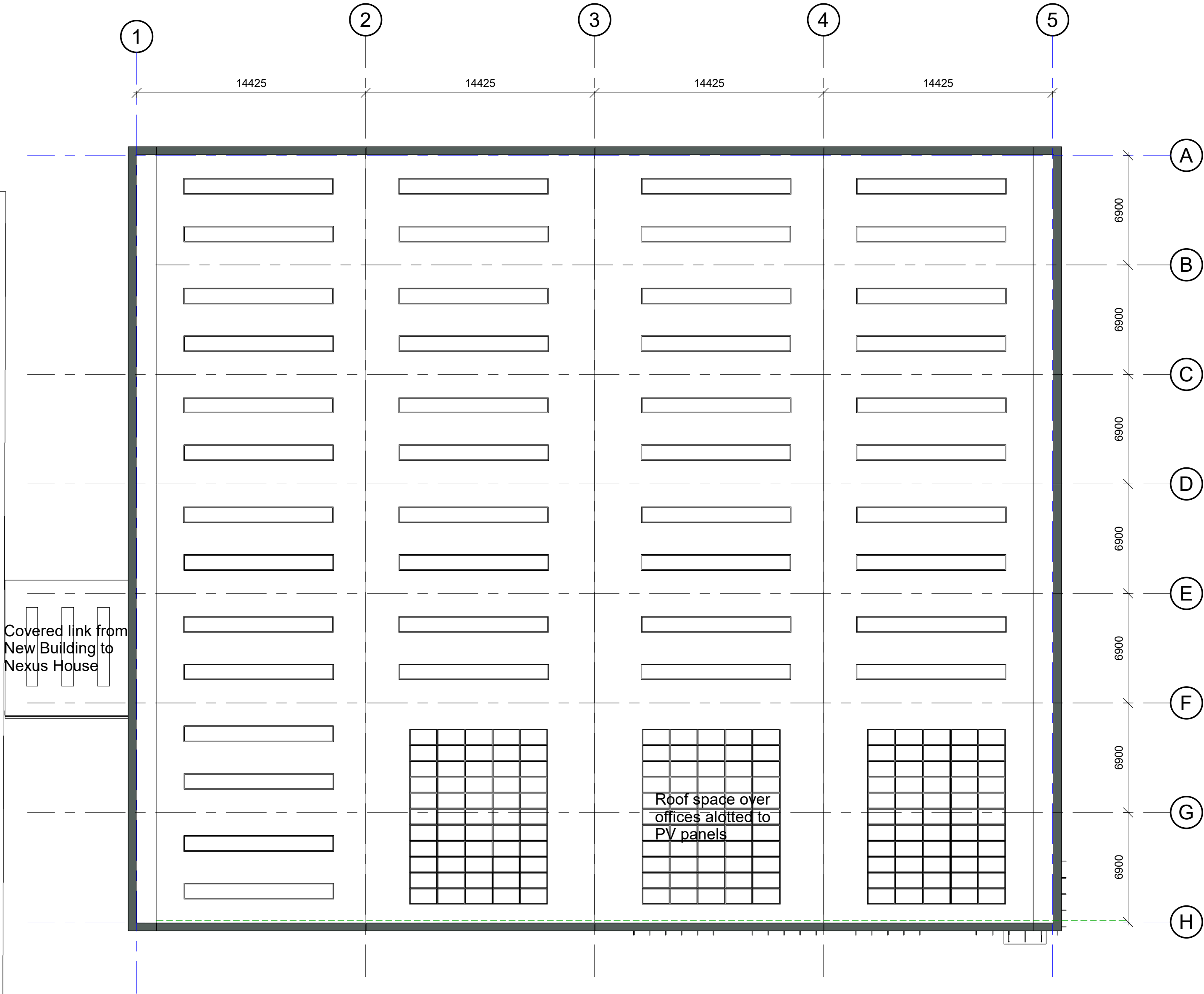
Roof Level Plan 1 : 200
