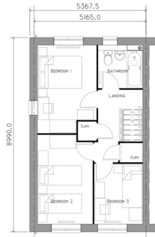
FIRST FLOOR PLAN GFA 40.31M2 (39.52M2)
