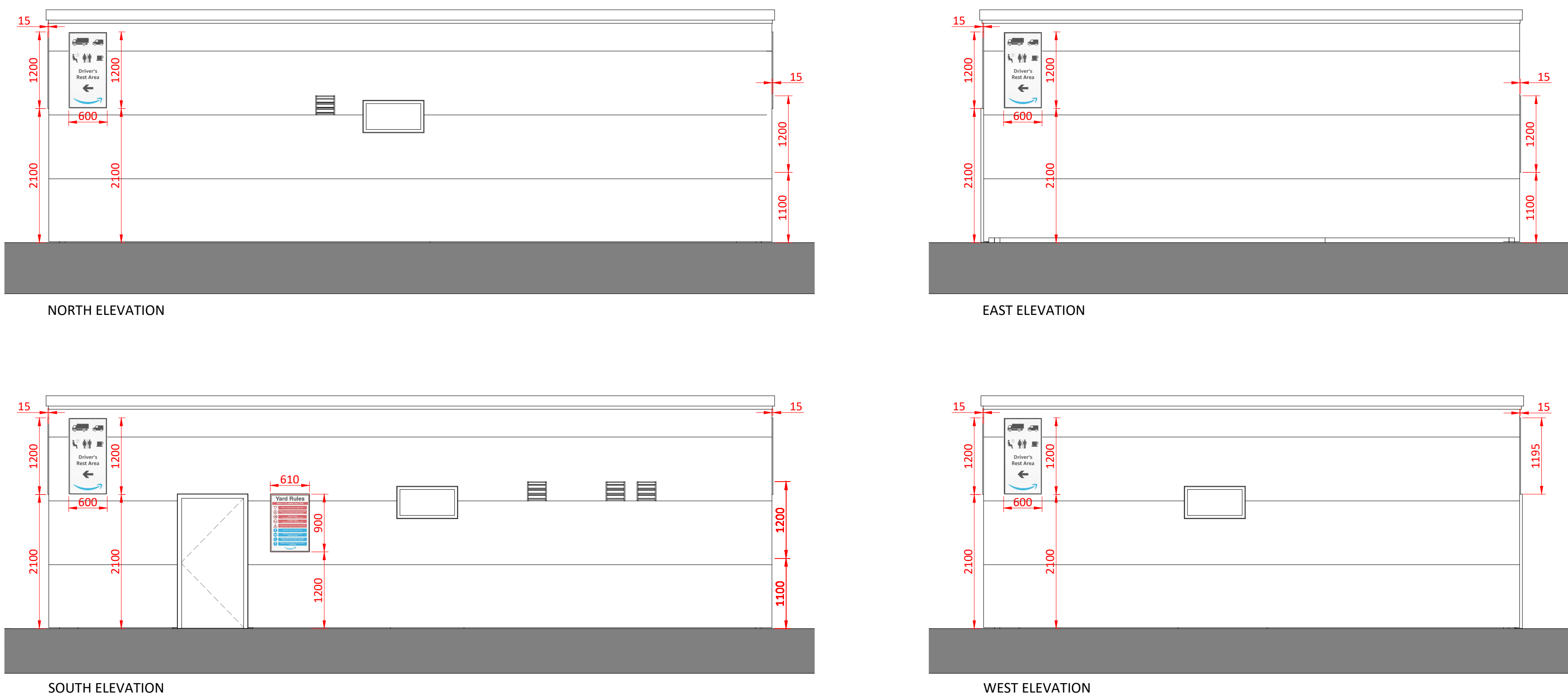
PROPOSED ELEVATIONS OF WELFARE BLOCK 1:50
