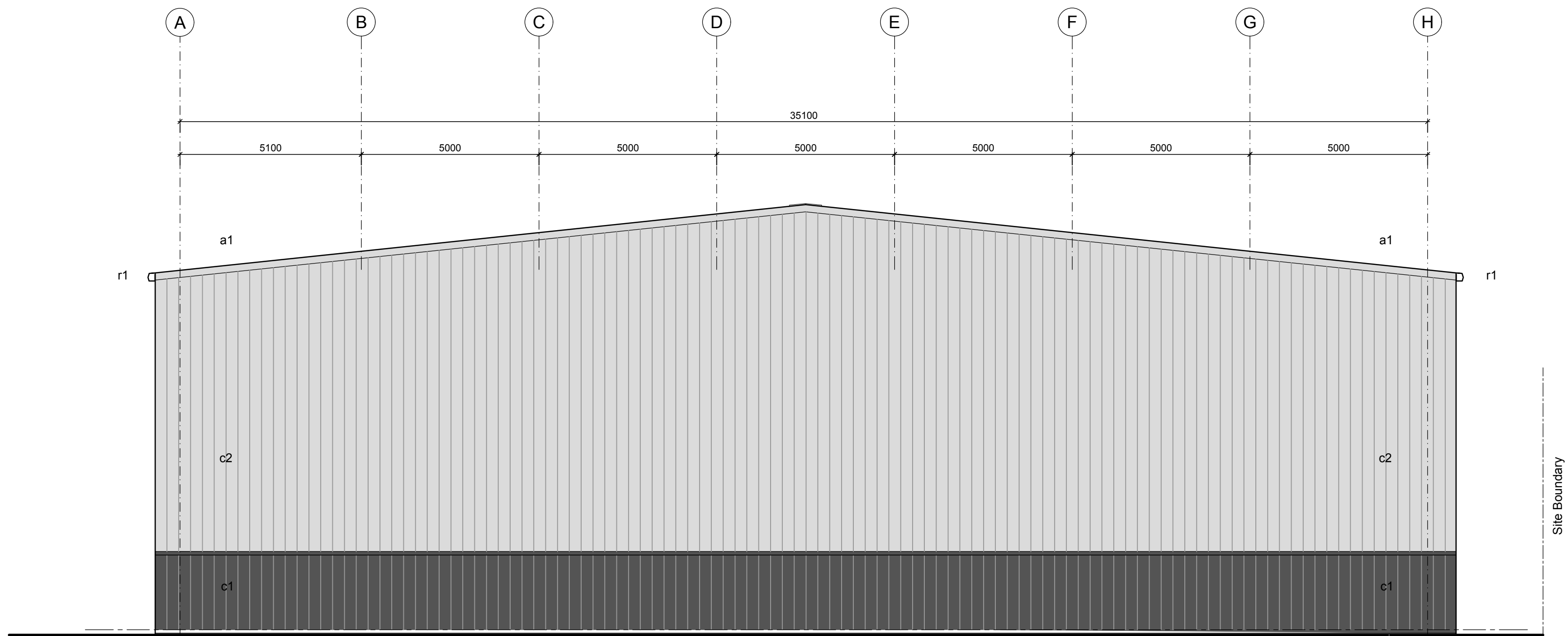
3. Side Elevation
