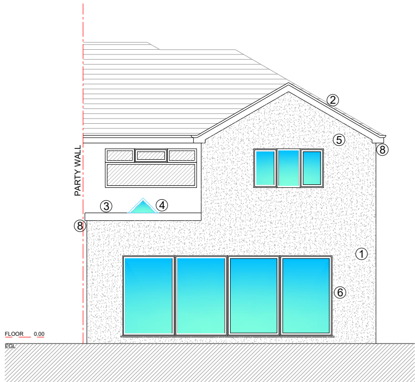
REAR ELEVATION
