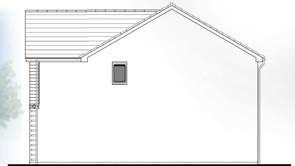
SIDE ELEVATION
