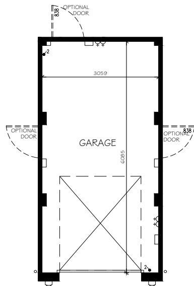
SINGLE GARAGE PLAN
