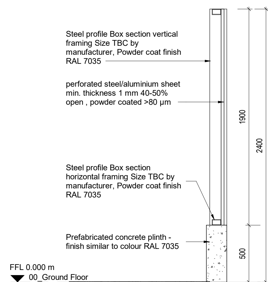
Section A - Mesh fencing panel Typical Section Scale @ 1 : 20
