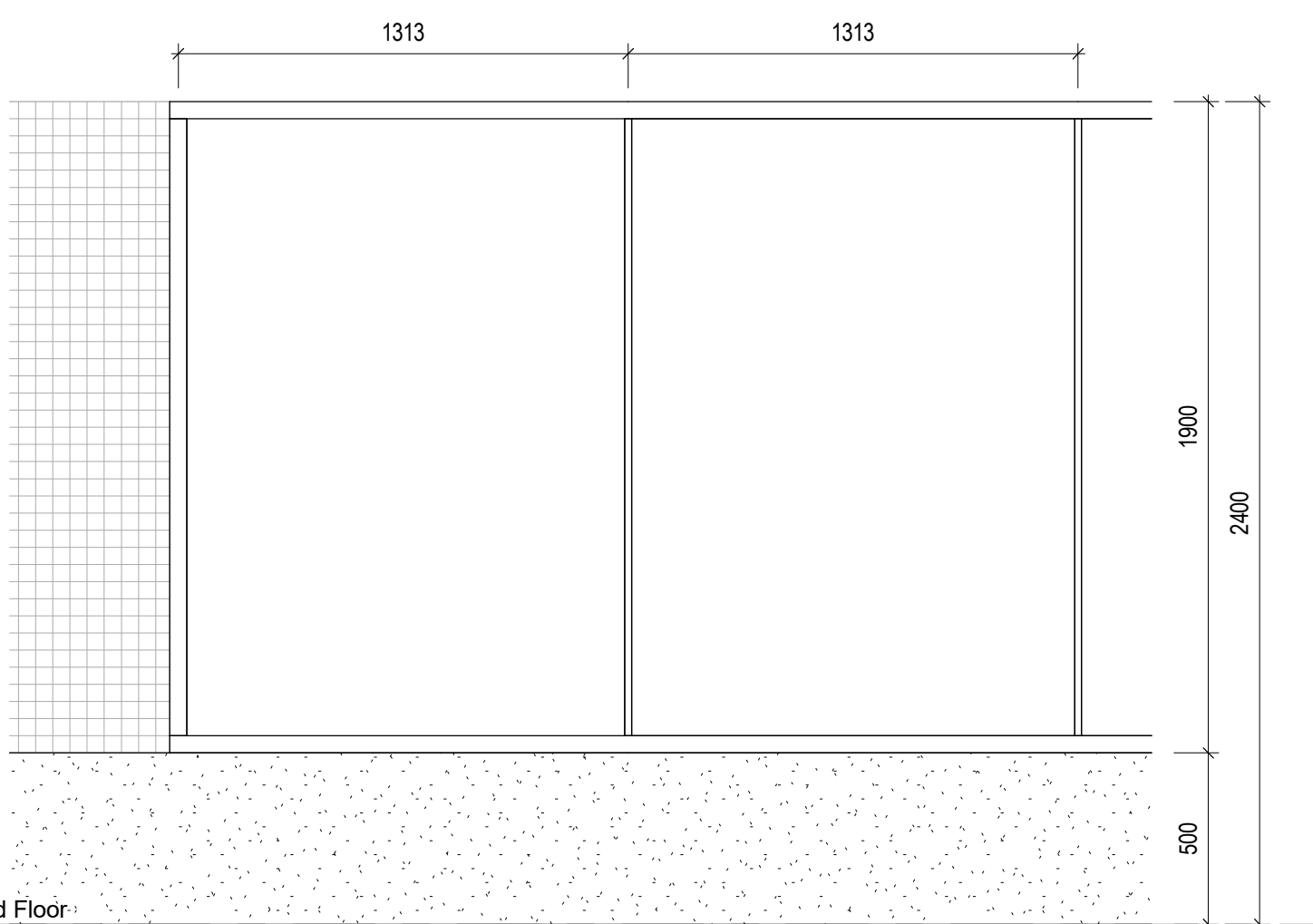
Glazed panel Typical Elevation Scale @ 1 : 20
