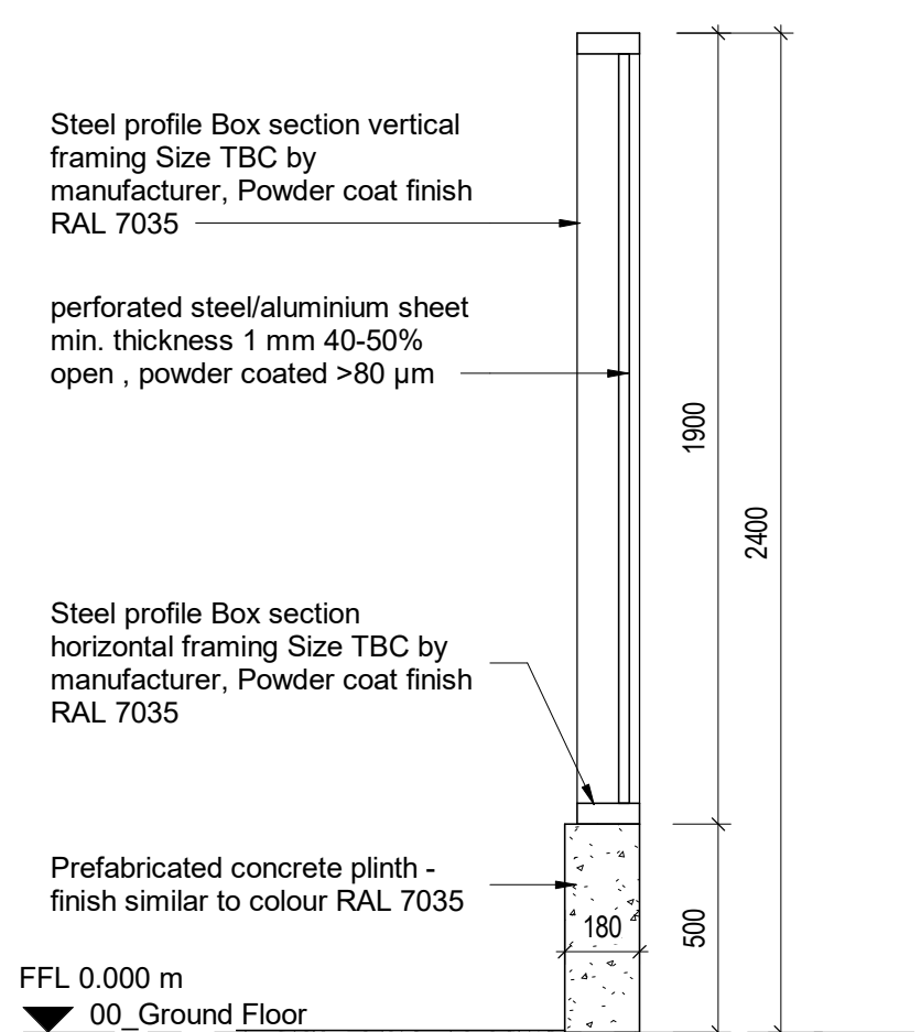
Section B - Glazed Panel Typical Section Scale @ 1 : 20
