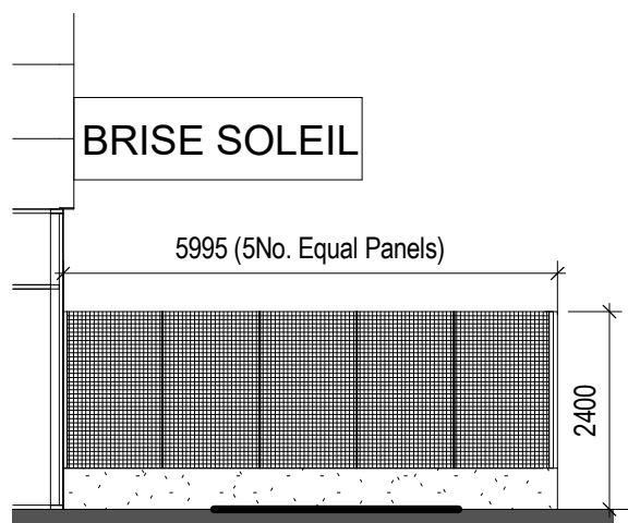
Ext Breakroom Elev A Scale @ 1 : 100
