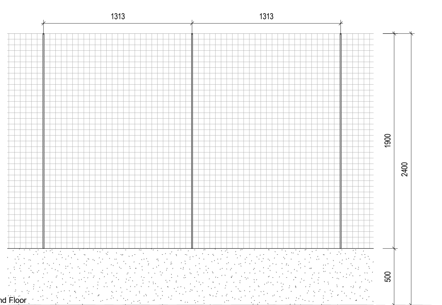
Mesh fencing panel Typical Elevation Scale @ 1 : 20
