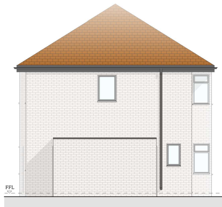
Existing Side Elevation (No. 16) 1 : 100
