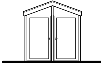
PROPOSED FRONT ELEVATION 1:100
