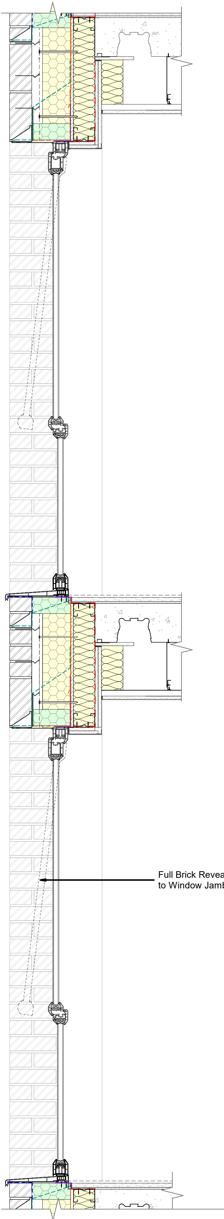
Window Full Height Section 1 : 10
