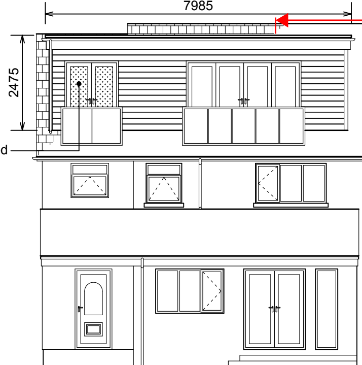
REAR ELEVATION AS PROPOSED
