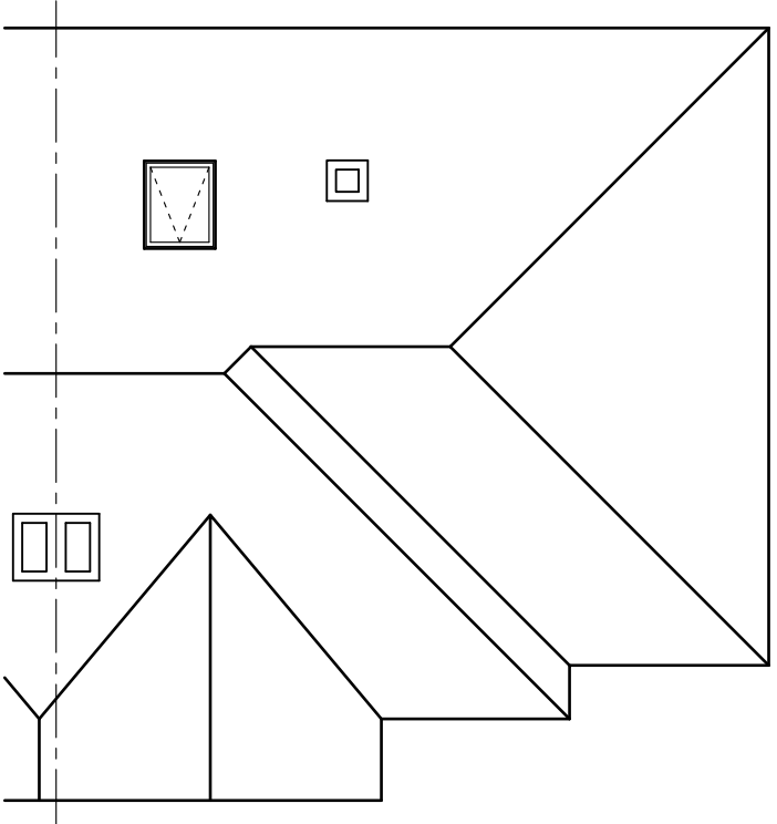
ROOF PLAN AS EXISTING
