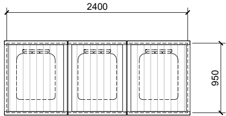
Proposed Bin Storage Plan @ 1:50
