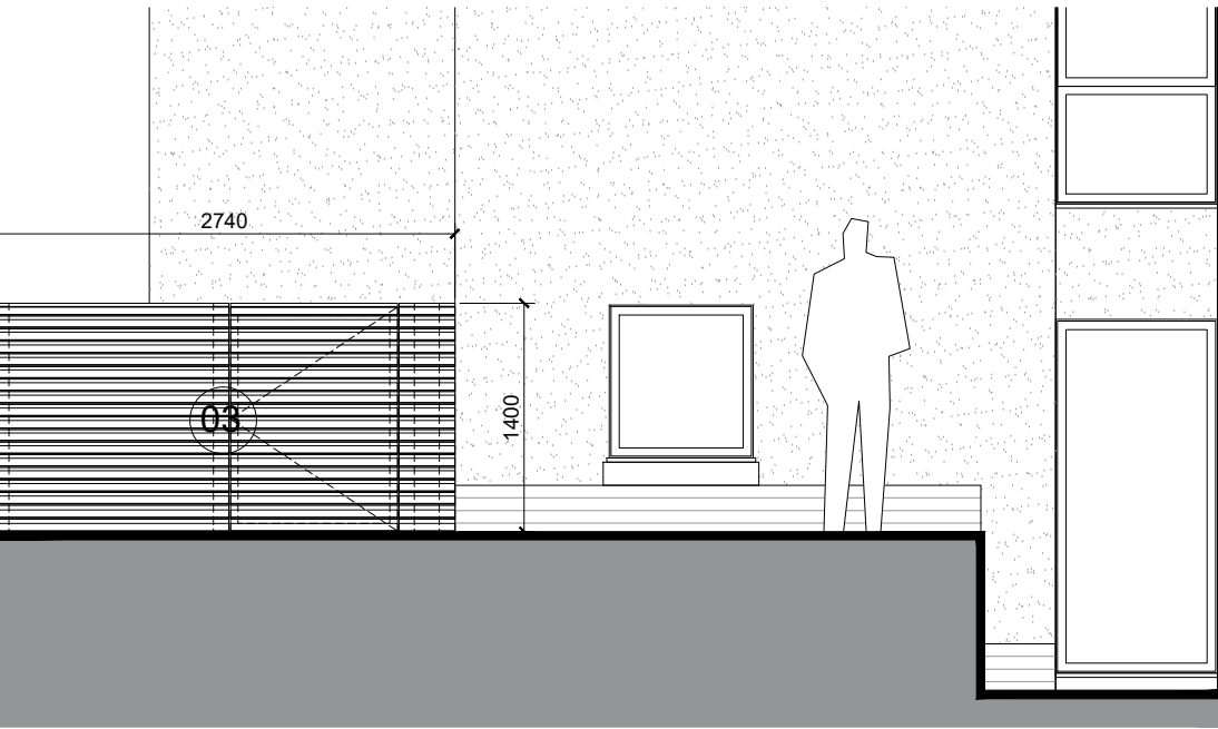
Proposed Front Fence Panel & Gate Elevation @ 1:50
