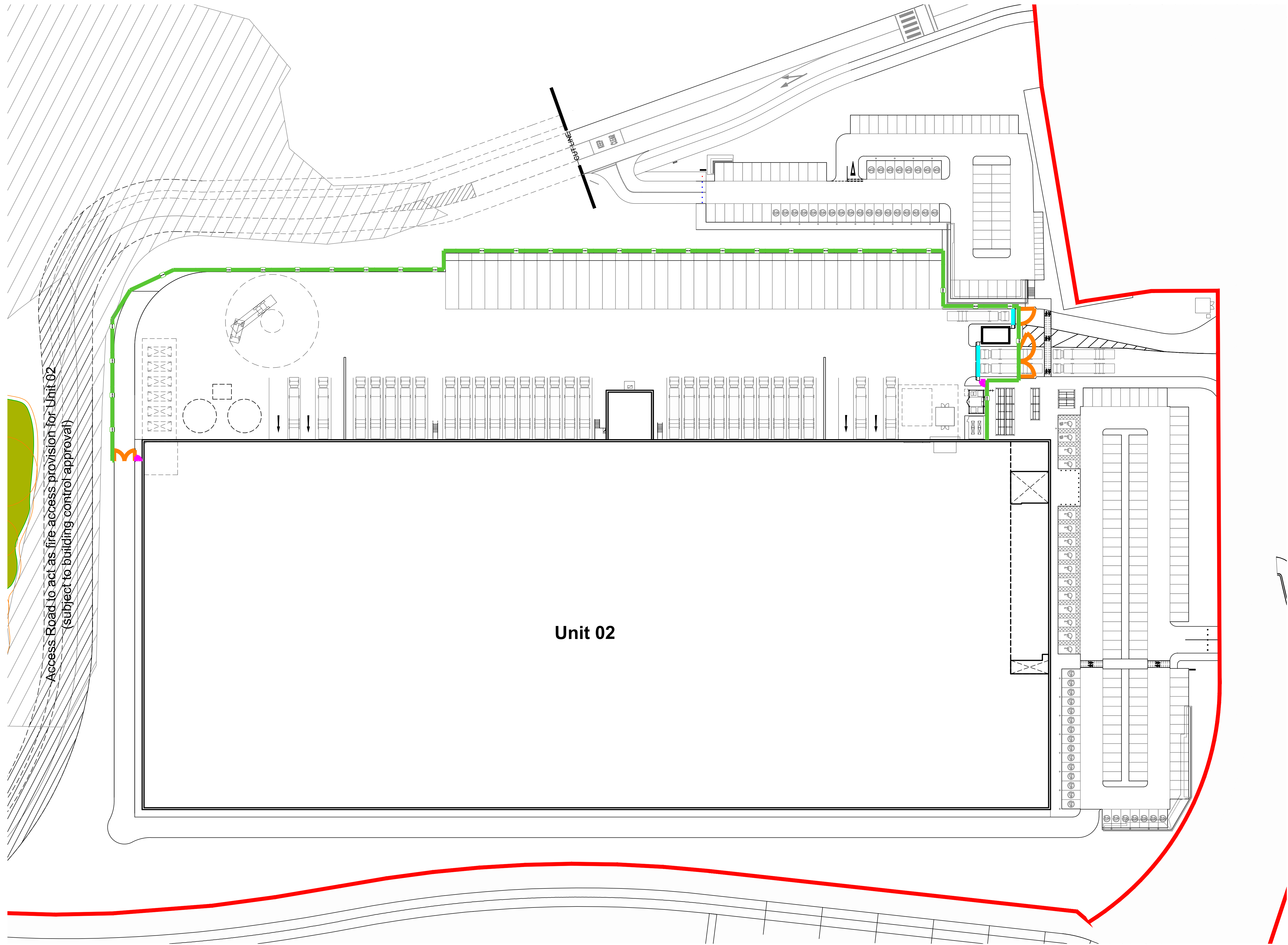
Fencing Plan Scale 1:500
