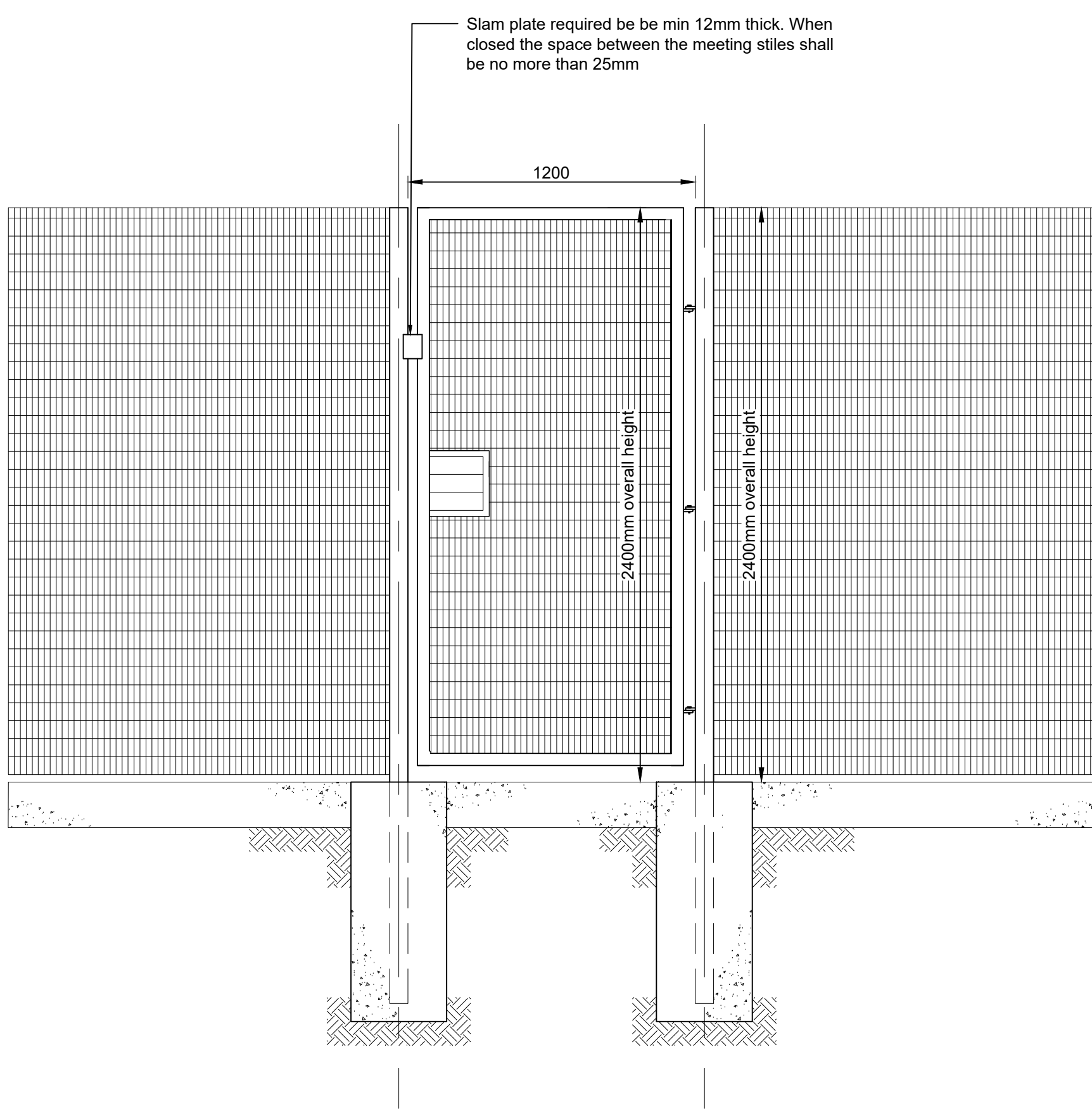
Personnel Gate Details Scale 1:20
