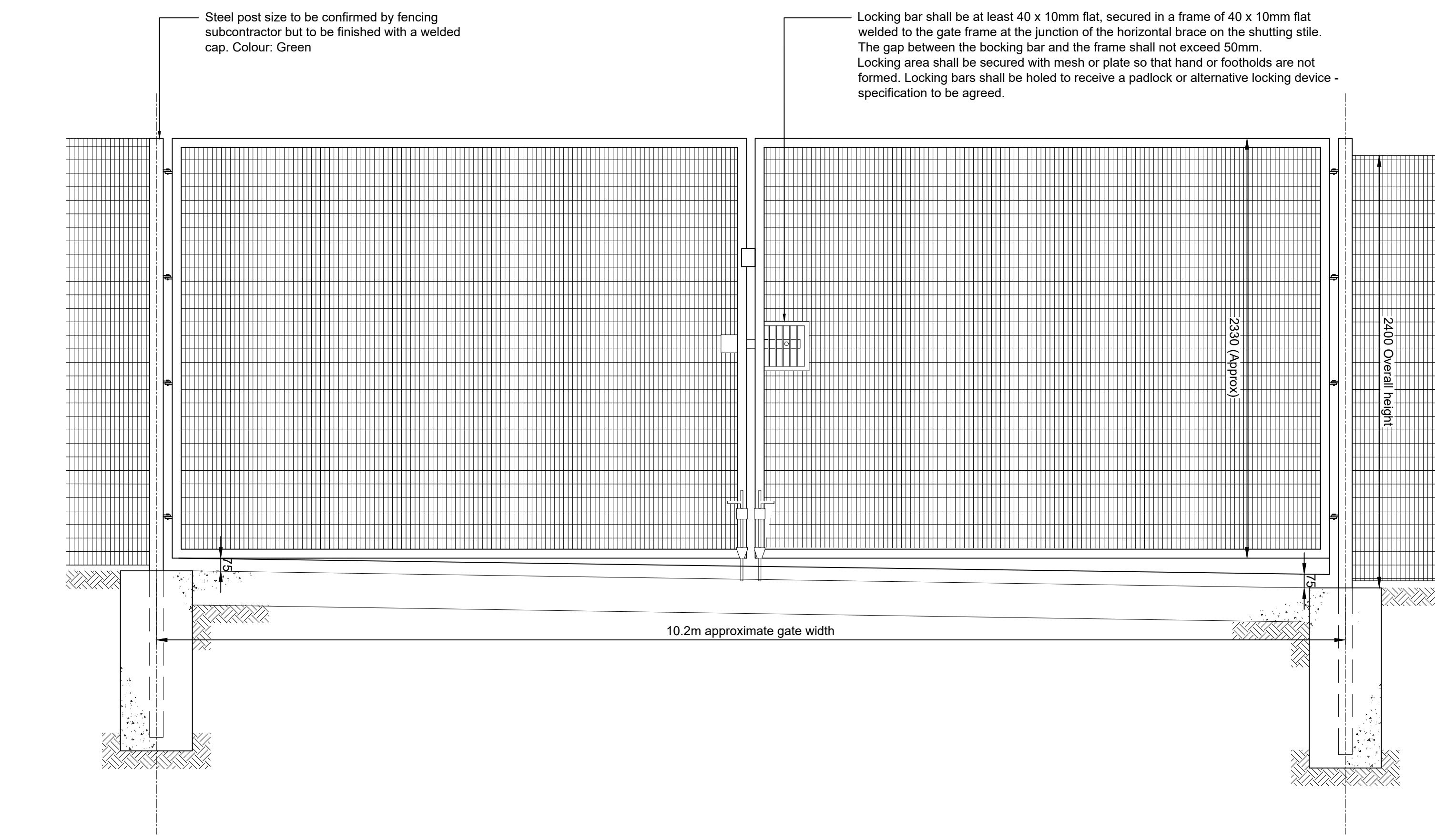
Security Access Gate Details Scale 1:20
