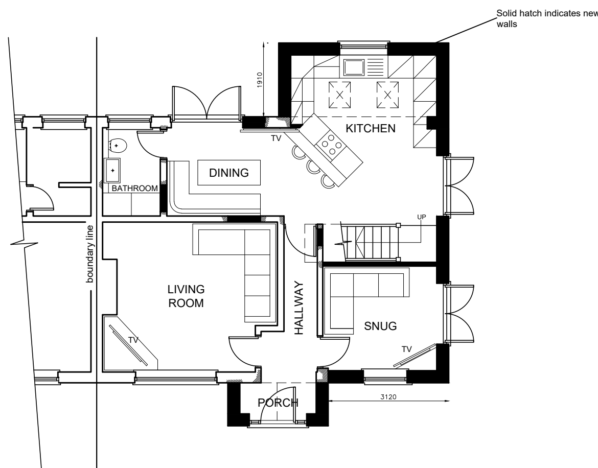
GROUND FLOOR
