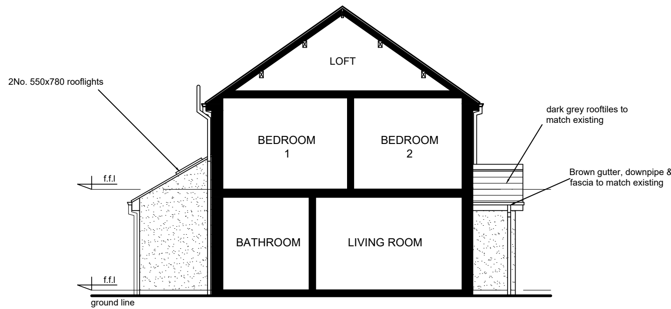
LEFT ELEVATION
