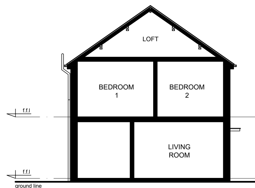
LEFT ELEVATION
