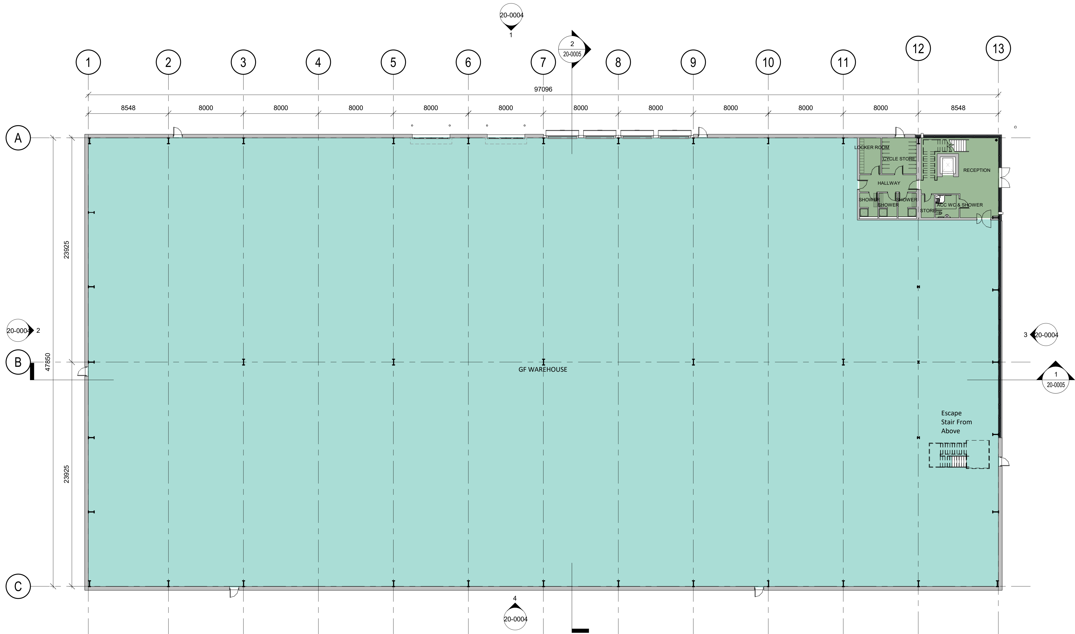
Ground Floor GA Plan 1 : 200
