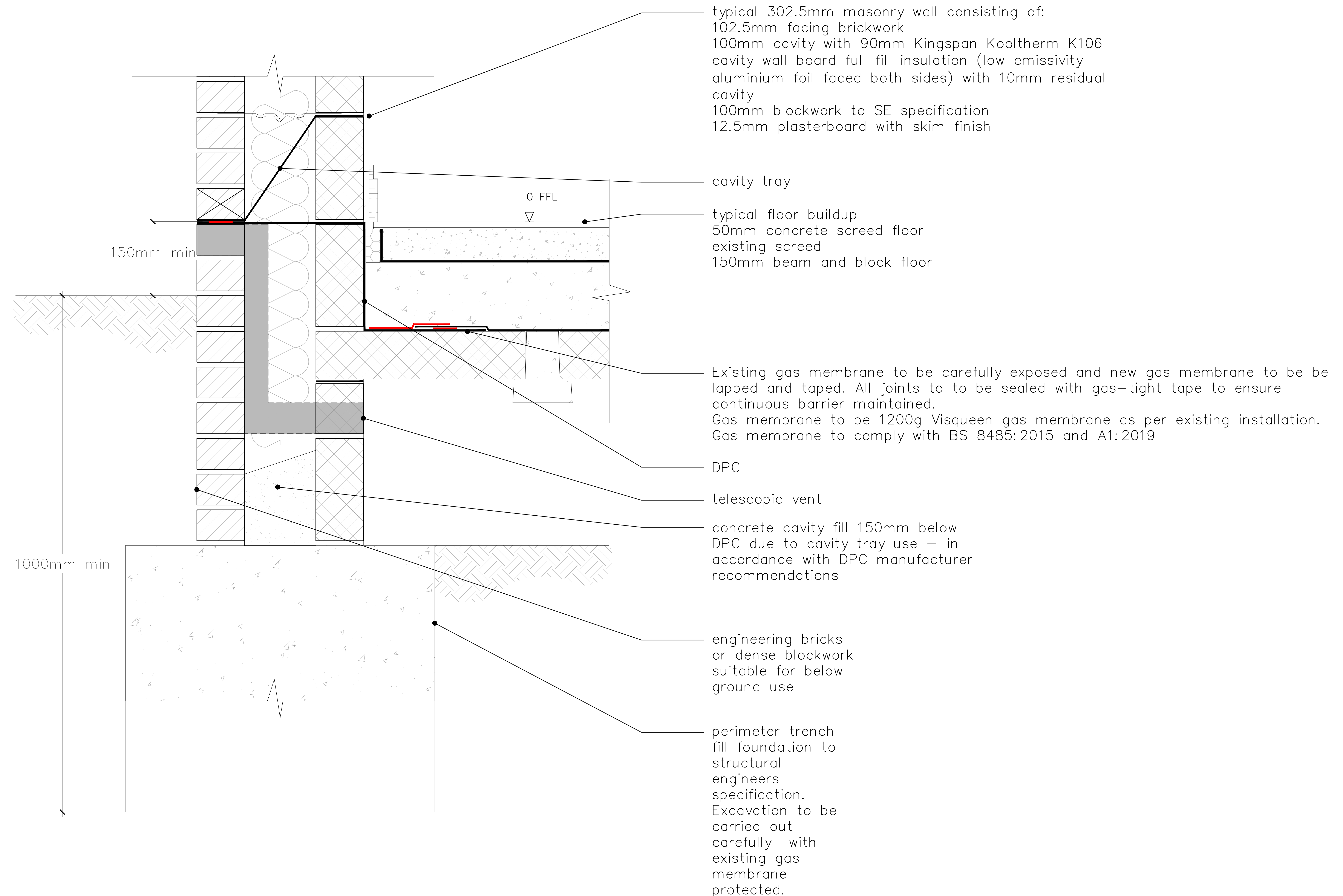
Foundation Detail
