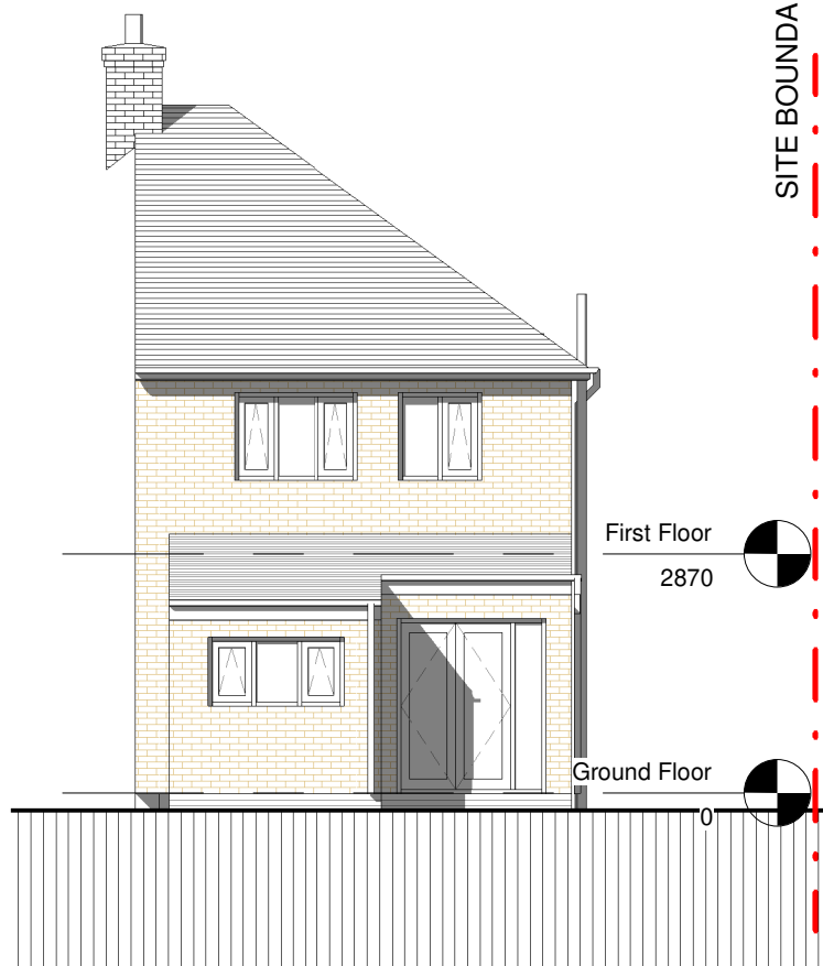
Rear Elevation 1 : 100
