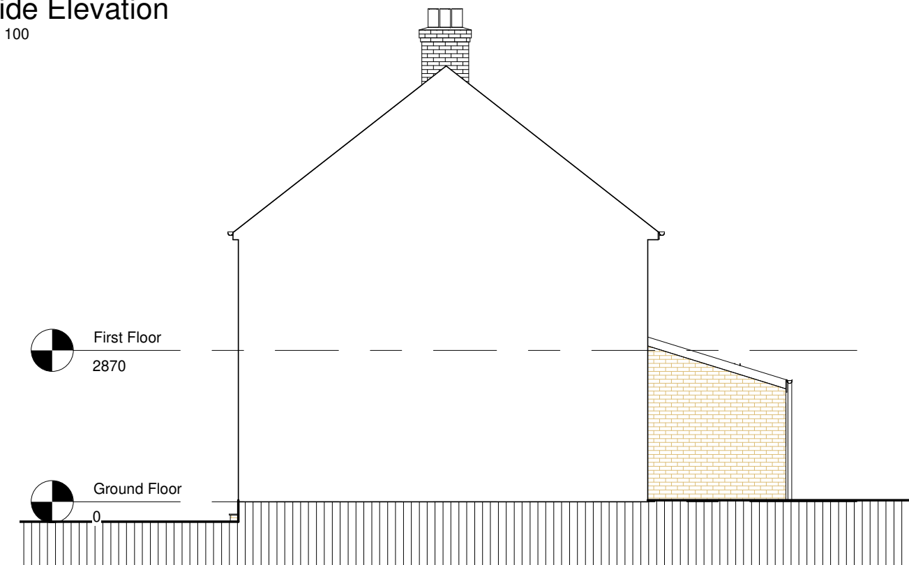
Elevation to No34 1 : 100
