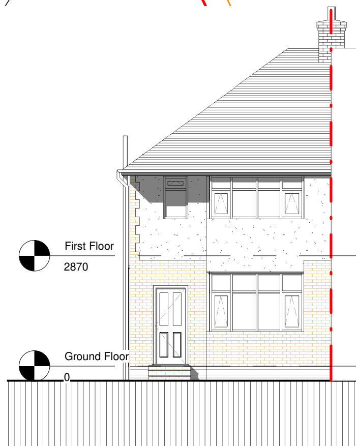
Front Elevation 1 : 100
