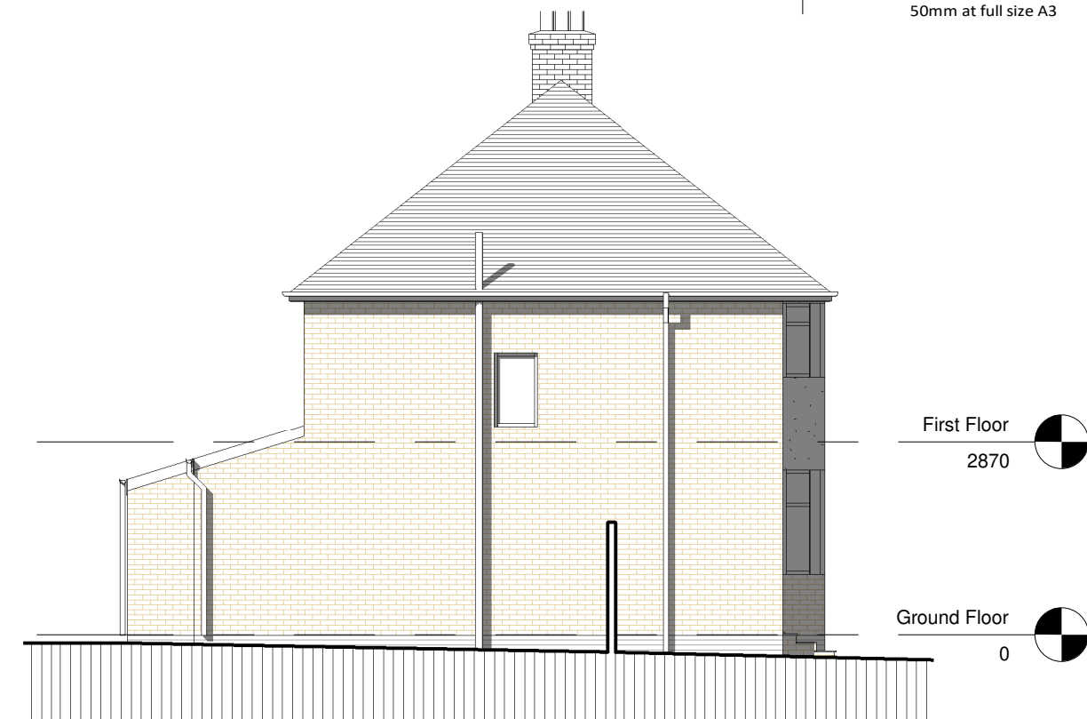
Side Elevation 1 : 100
