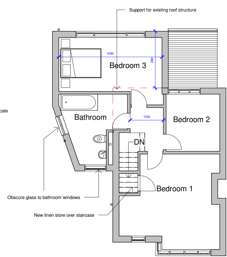
First Floor 1 : 100
