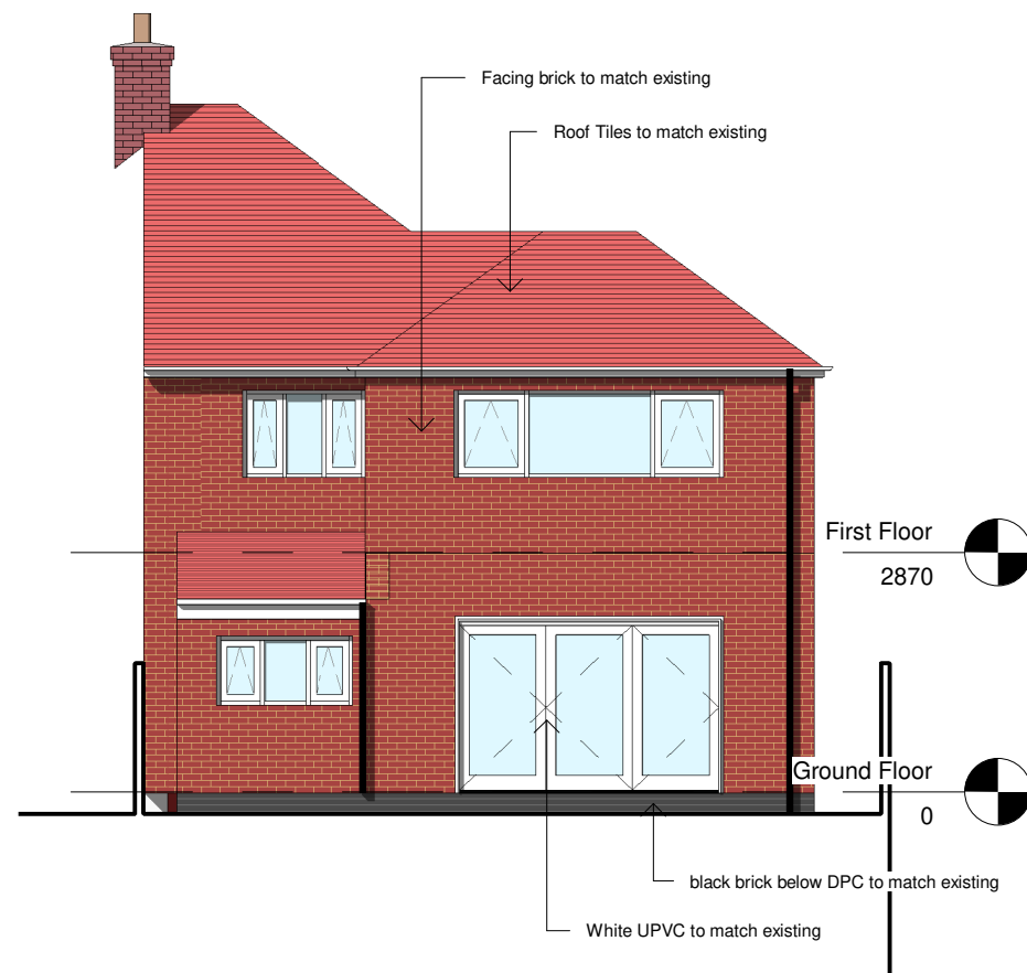
02 Rear Elevation 1 : 100
