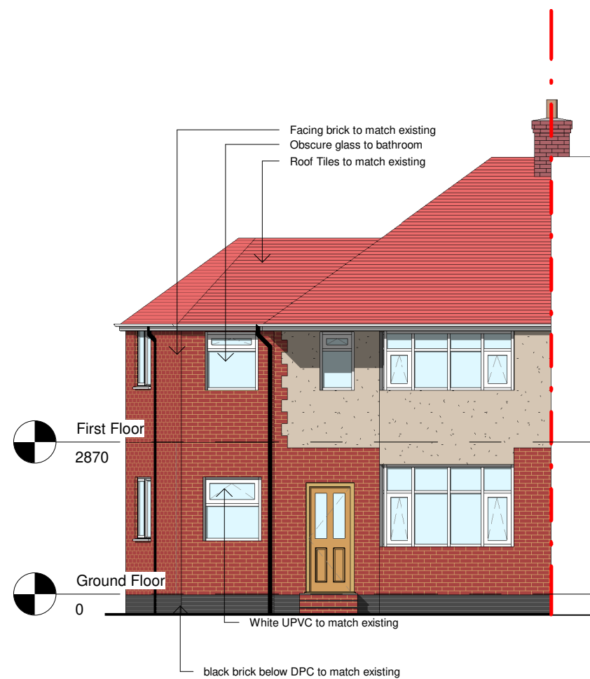
01 Front Elevation 1 : 100
