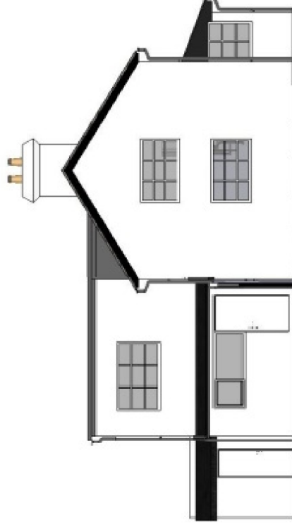
Proposed Right Elevation Scale: 1:100
