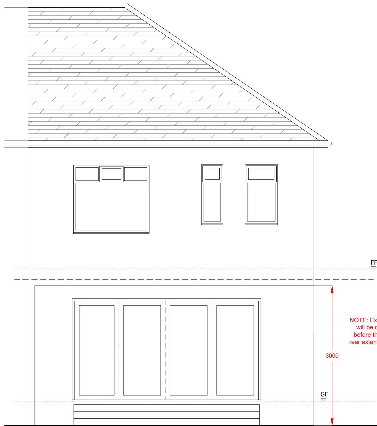
Proposed Rear Elevation 1:50
