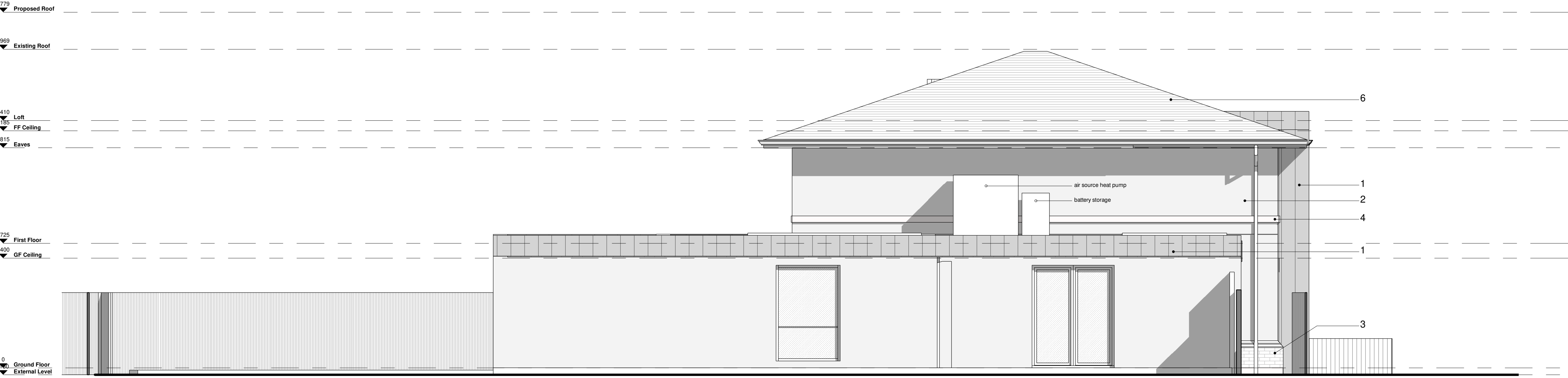
2 Proposed Elevation Side 2 Scale: 1 : 50
