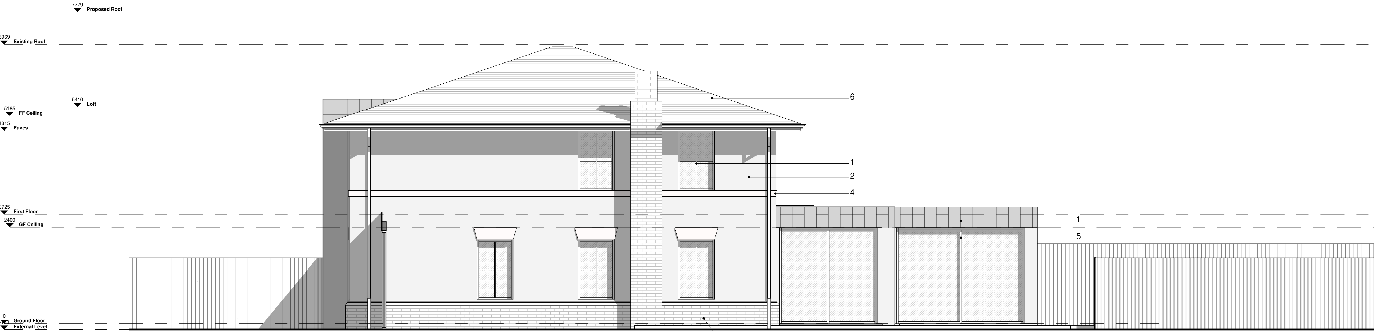
1 Proposed Side Elevation Scale: 1 : 50
