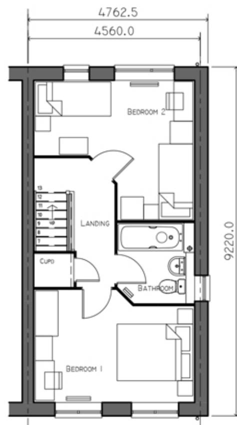
FIRST FLOOR PLAN GFA 36.27M 2 (35.51M 2 )
