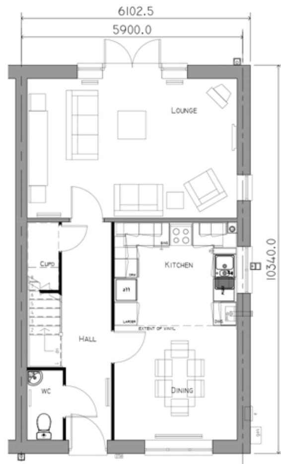
GROUND FLOOR PLAN GFA 53.96M 2 (53.05M 2 )
