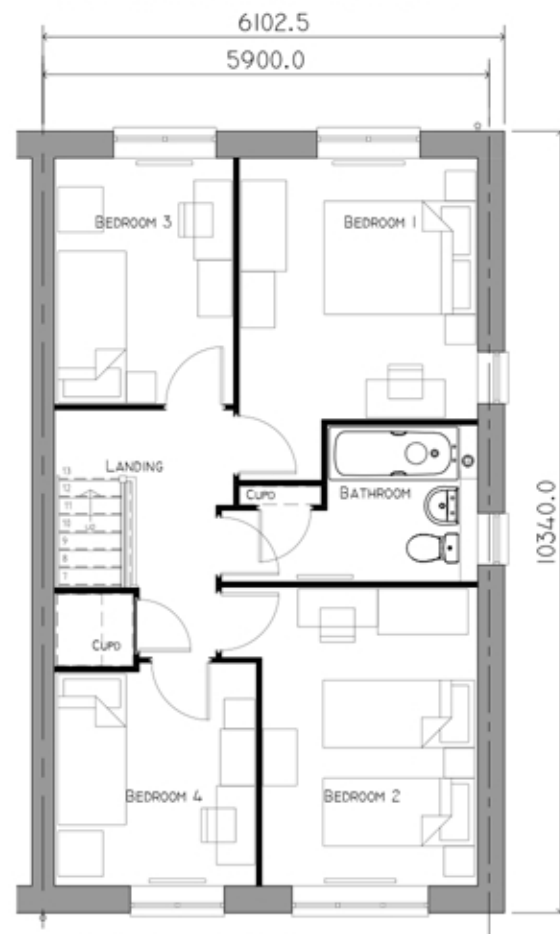
FIRST FLOOR PLAN GFA 53.96M 2 (53.05M 2 )
