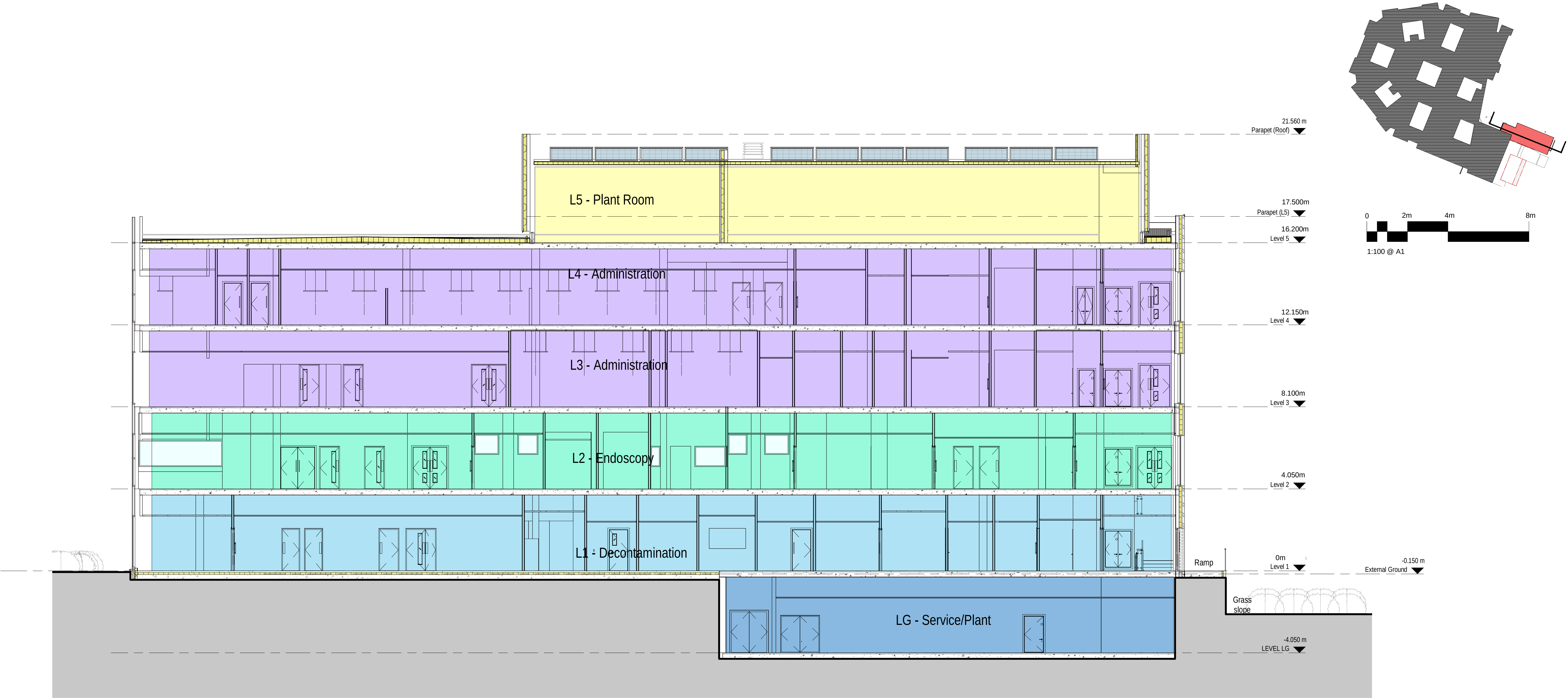
Typical Proposed Section (Long)
