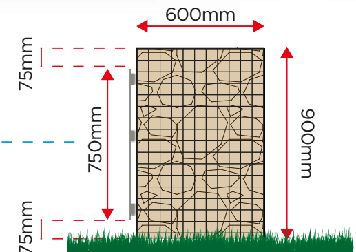
Gabion wall side view
