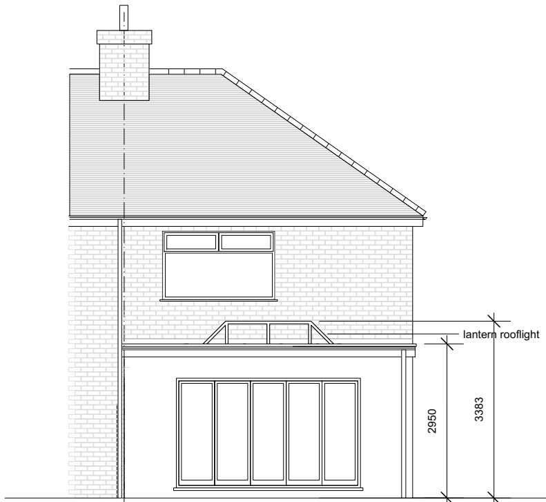
Proposed East Elevation
