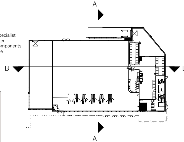
SS Key Plan SS 1:1000
