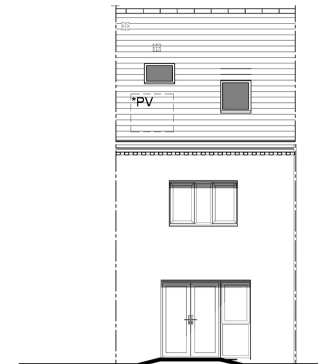
REAR ELEVATION
