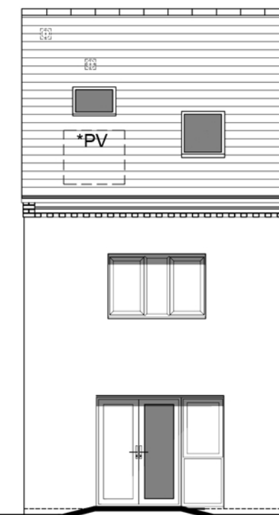
SIDE ELEVATION
