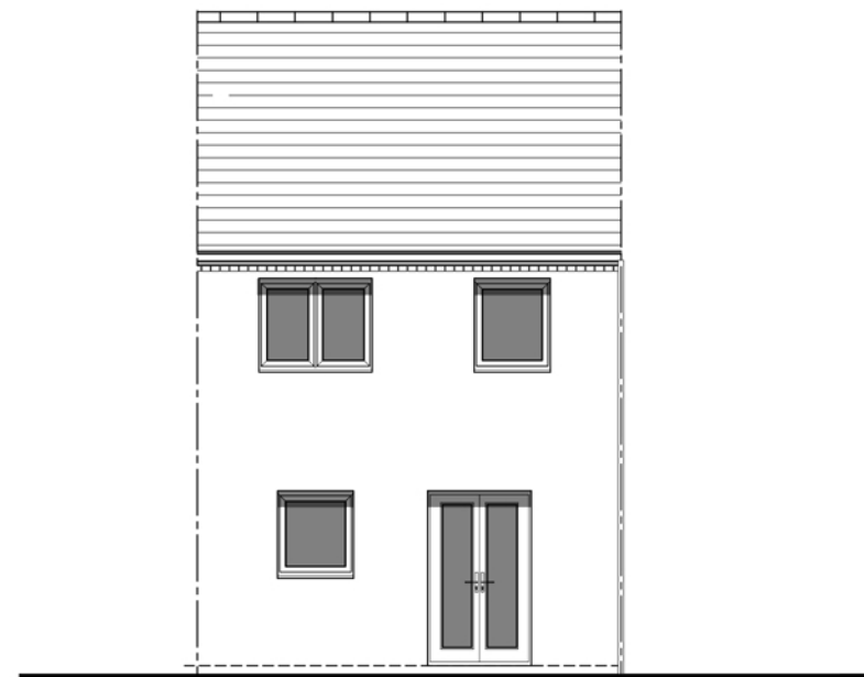
REAR ELEVATION
