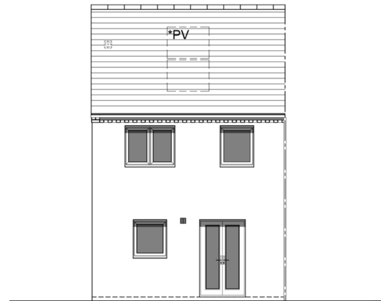
REAR ELEVATION
