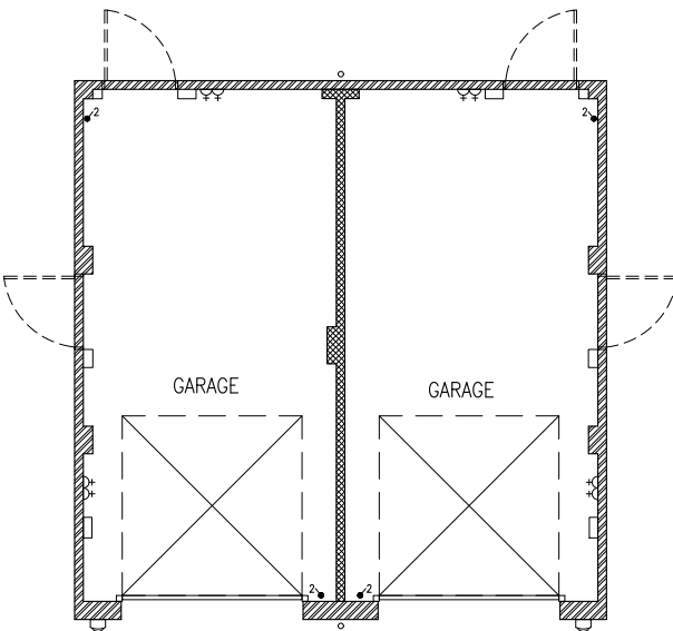
TWIN GARAGE PLAN
