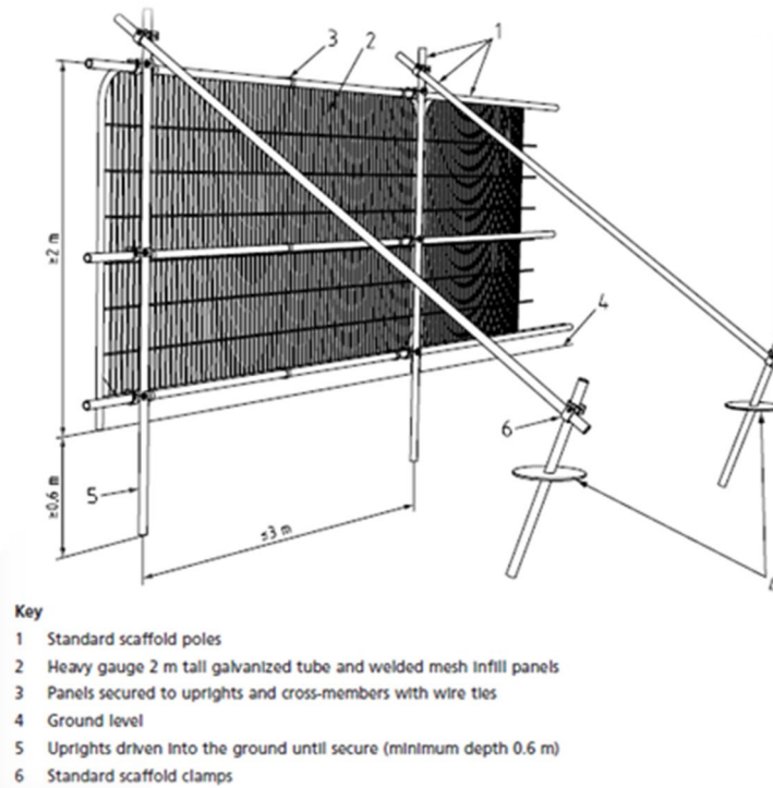
Figure 2: BS5837:2012 - Figure 2, Default specification for protective barriers.
