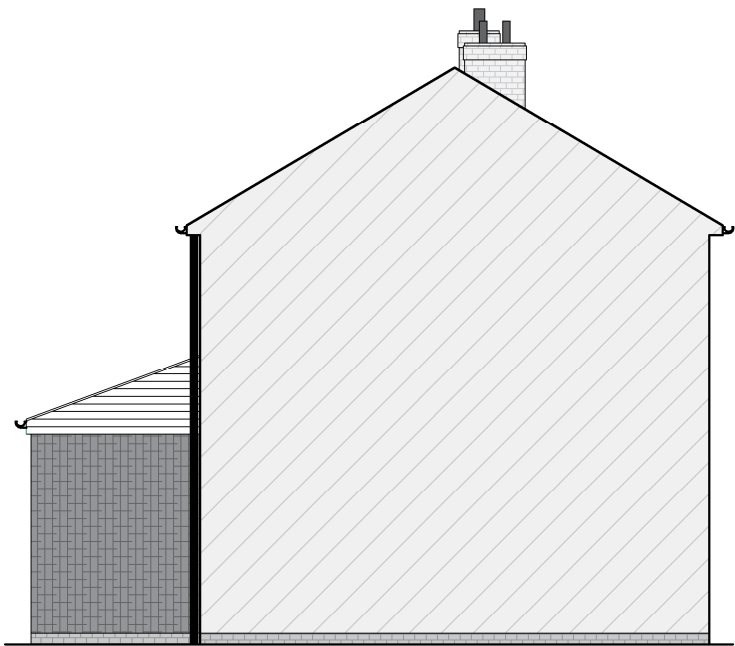
EXISTING REAR ELEVATION (Scale 1:100) SCALE BAR - (mm) 500 1000 2000
