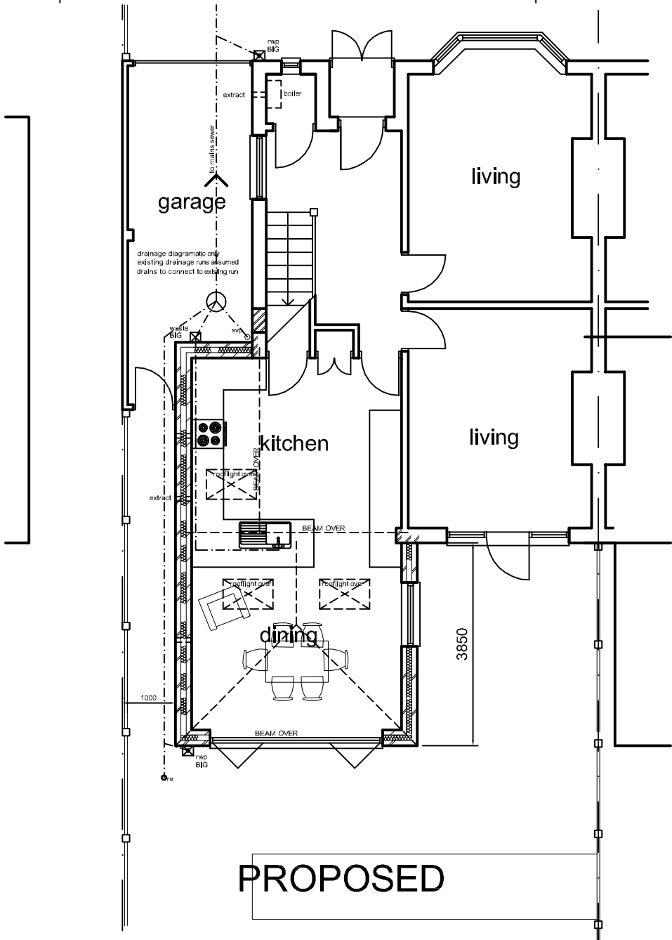
REAR PROPOSED
