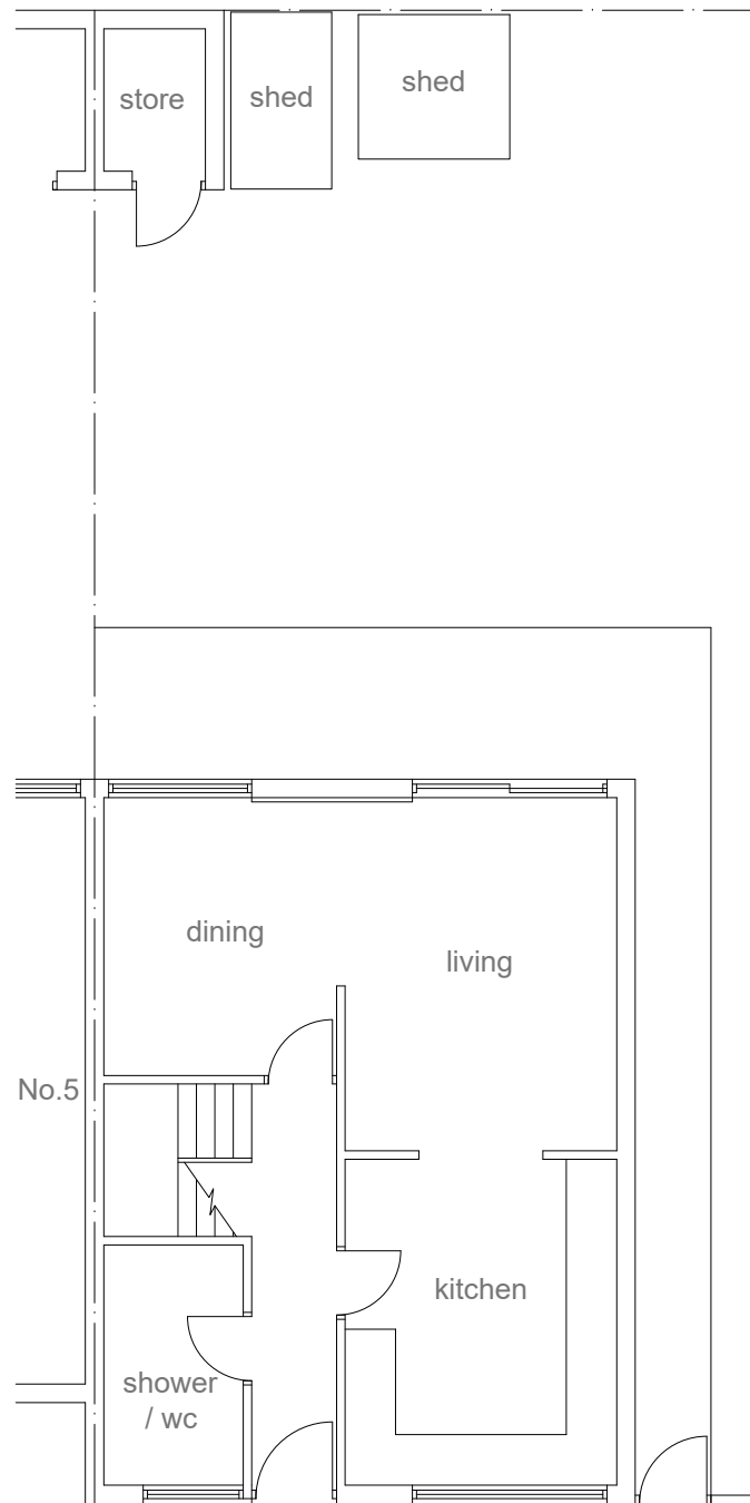
Existing ground floor plan and site plan @ 1:100 scale
