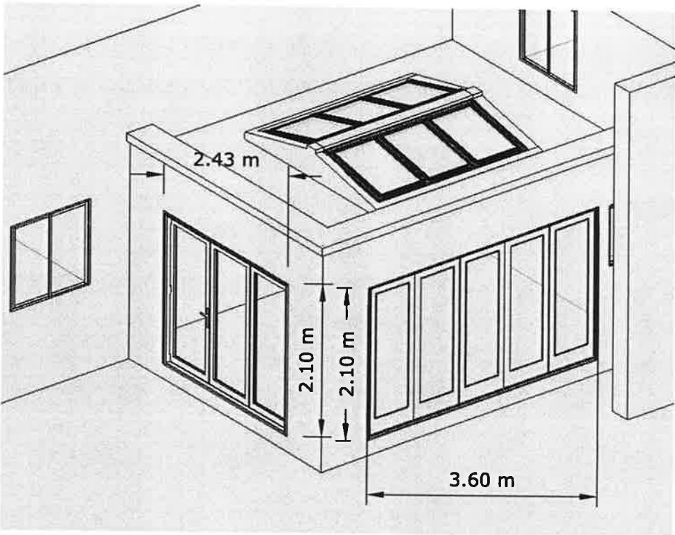
Iso with door openings
