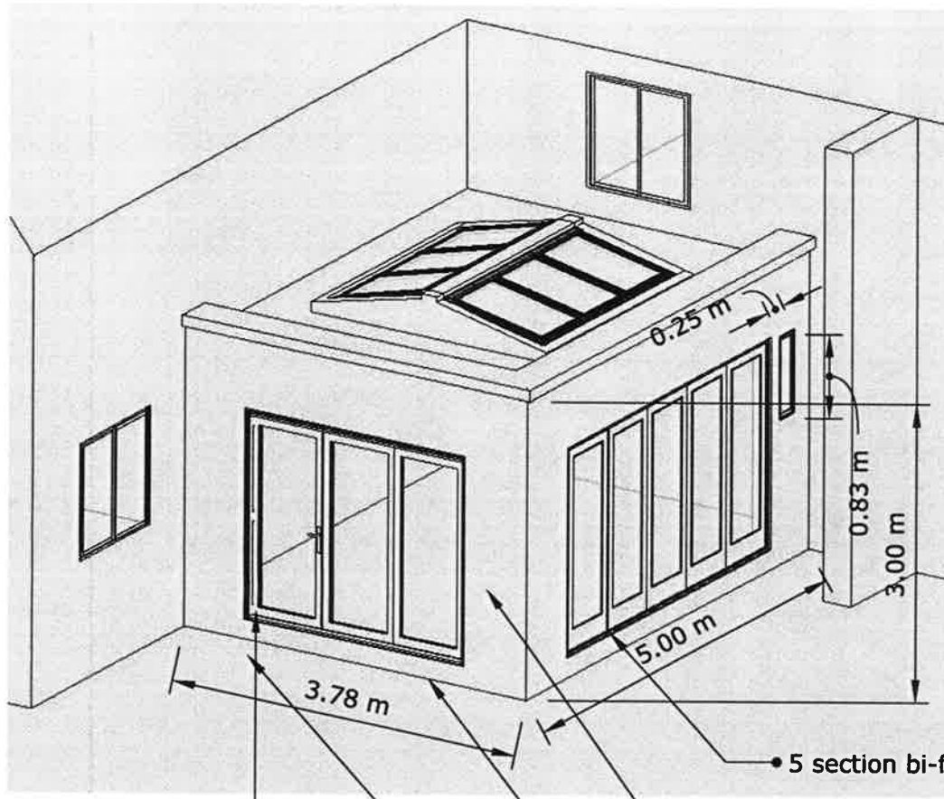
Isometric View
