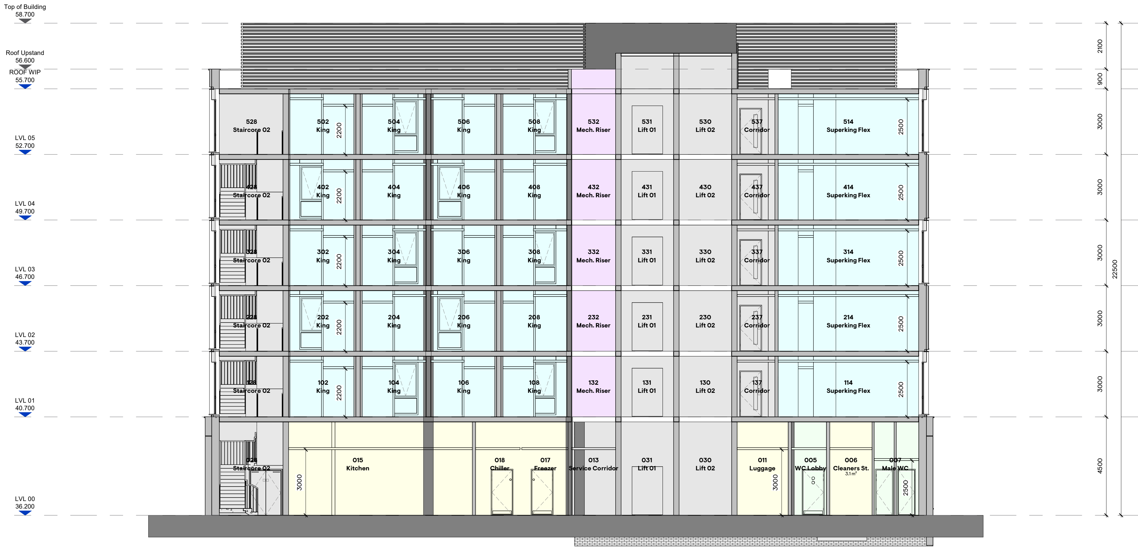
1 Section C-C Scale - 1 : 100
