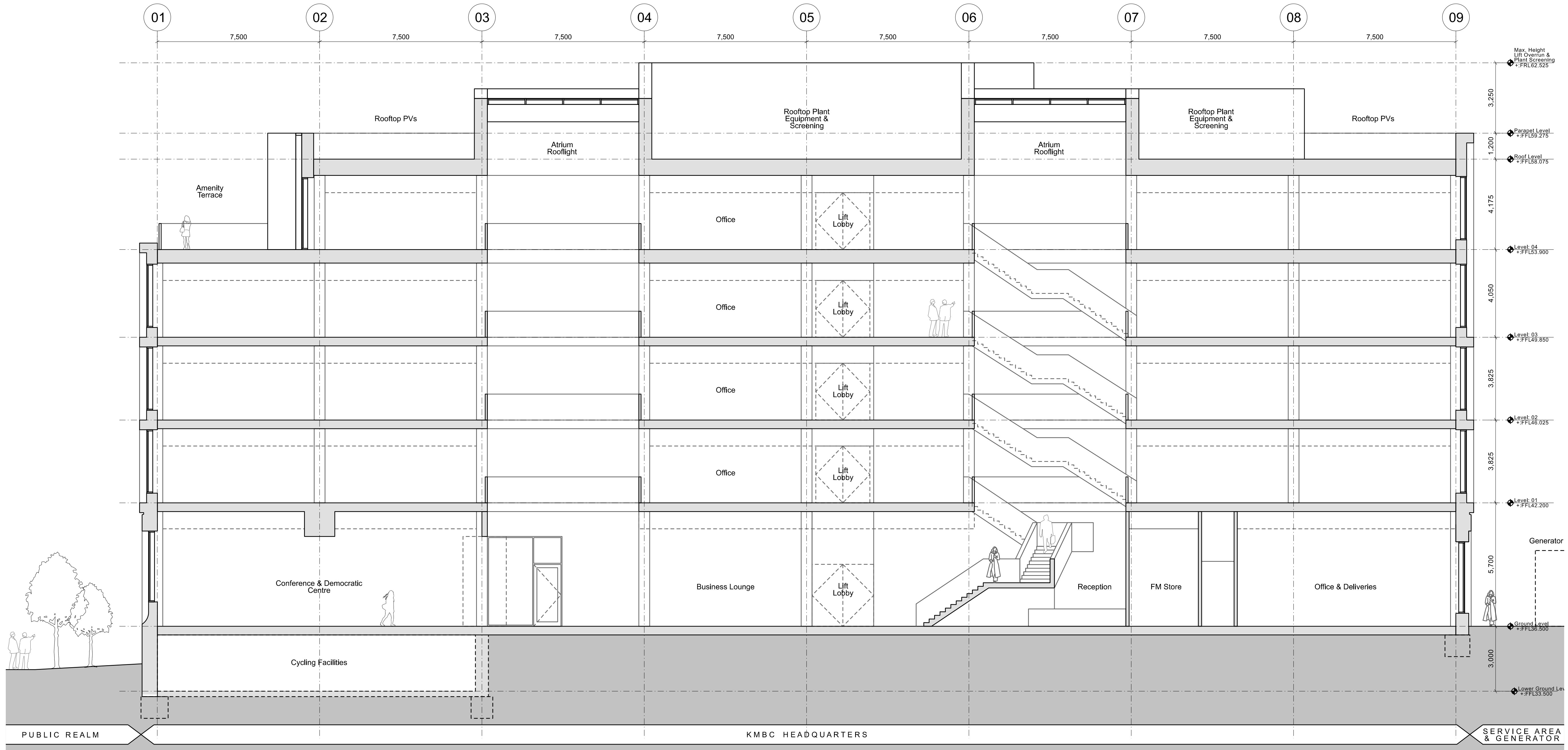
LONG SECTION AA
